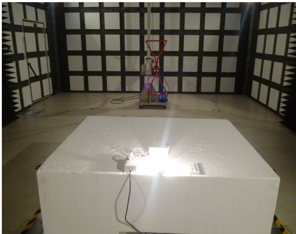
Radiated Emission -Rear View (Below 1GHz) Main
