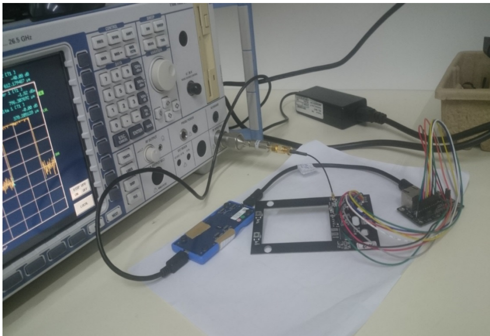
Conducted -Front View
