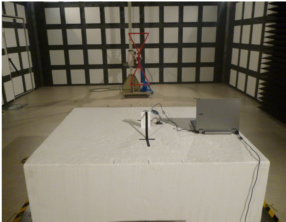
Radiated Emission -Rear View (Below 1GHz) Remote
