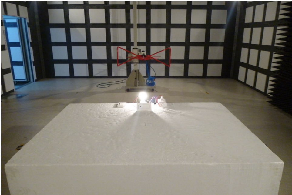
Radiated Emission -Rear View (Below 1GHz) Main
