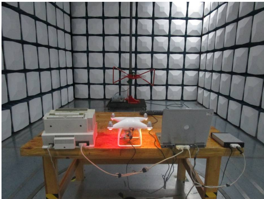
Radiated Emission Above 1GHz Rear View (Operating Mode)
