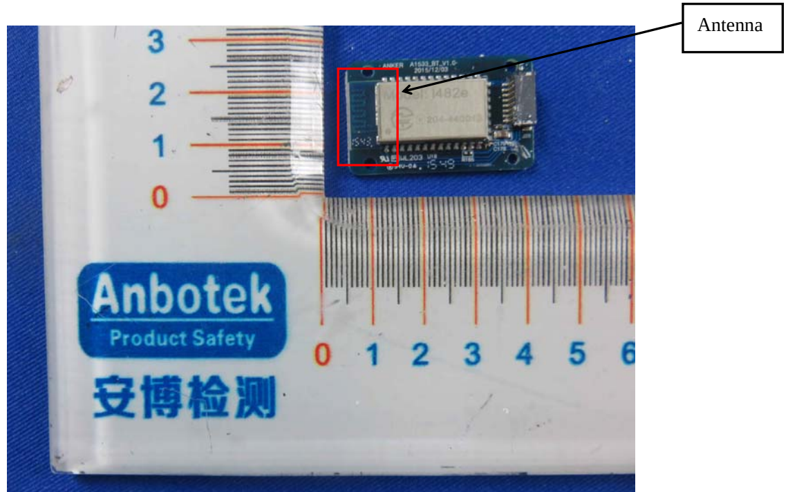
Figure 26 PCB of The EUT-Front View (With Shielding) (Bluetooth CSR8811)
