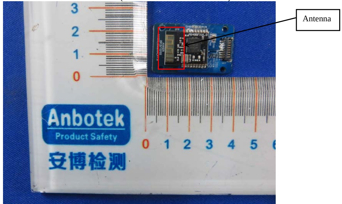
Figure 24 PCB of The EUT-Front View (Bluetooth N51822 iBeacon)
