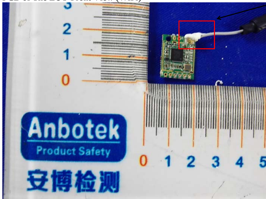
Figure 29 PCB of The EUT-Front View (WiFi)
