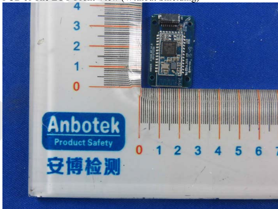
Figure 27 PCB of The EUT-Front View (Without Shielding)
