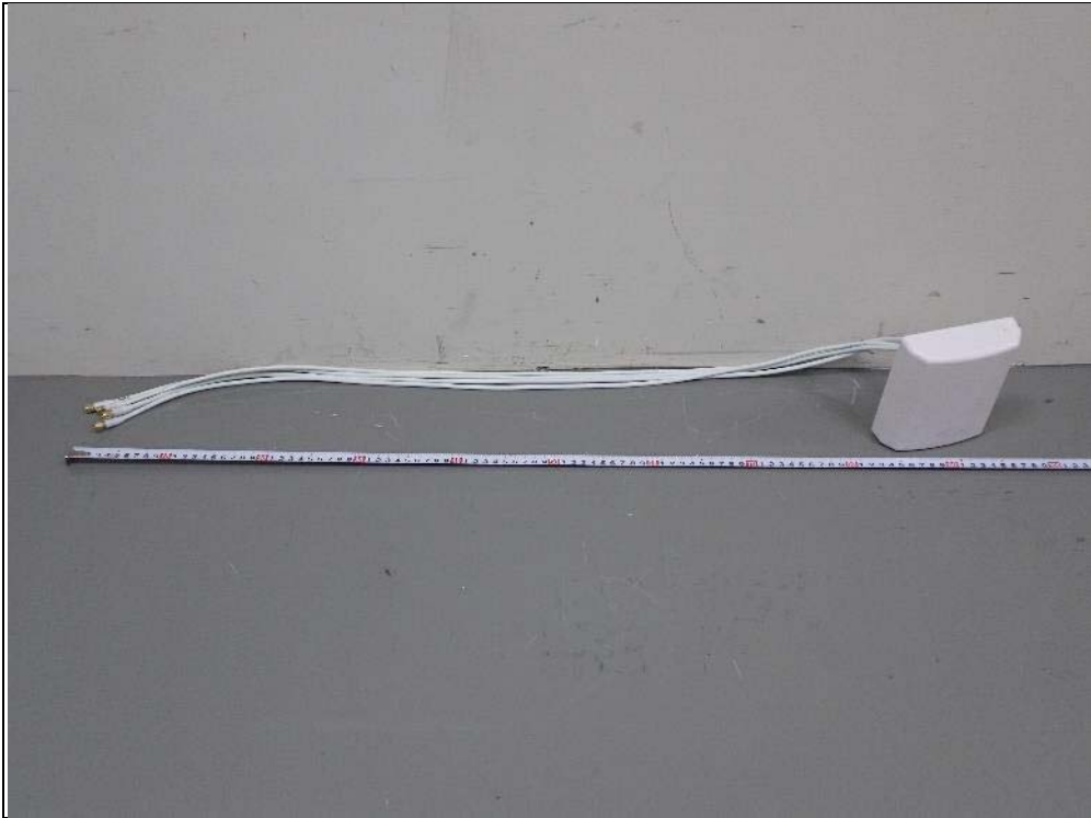
Ext WiFi PATCH Ant (Brand: AccelTex / Model: ATS-OP-245-810-4RPSP-36)
