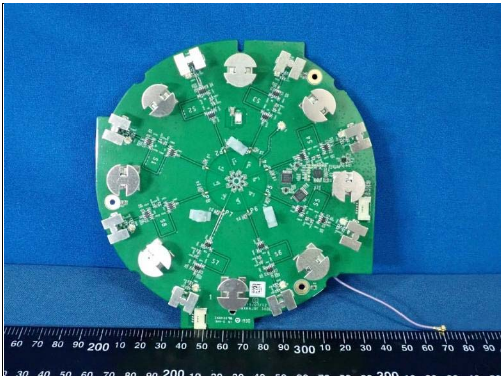
BT Array Antenna
