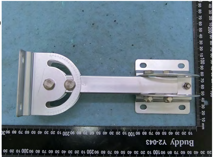
Antenna Bracket (Only for ant. 17 and ant. 19 use)
