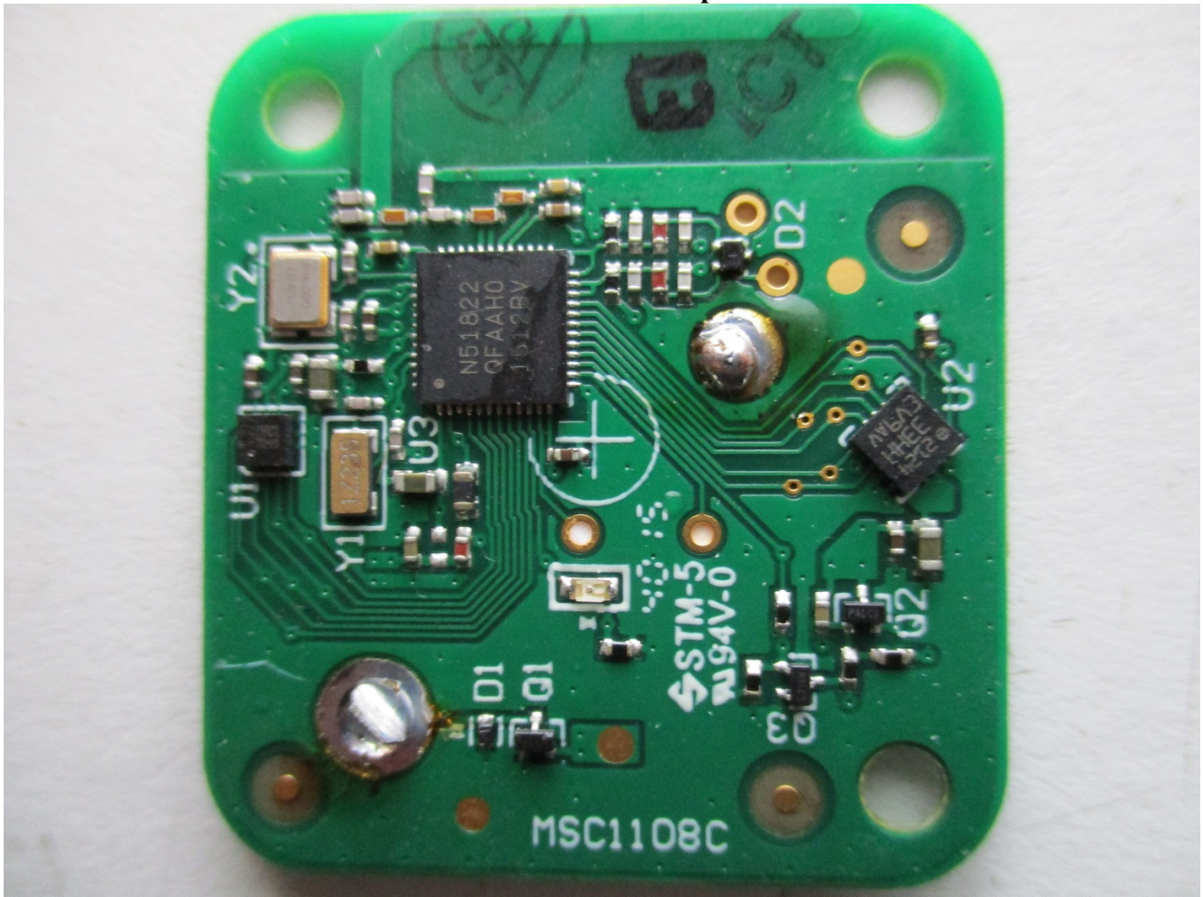
Circuit Board Top
