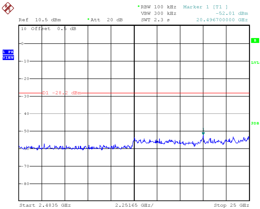
802.11g, Highest Channel, Plot B
