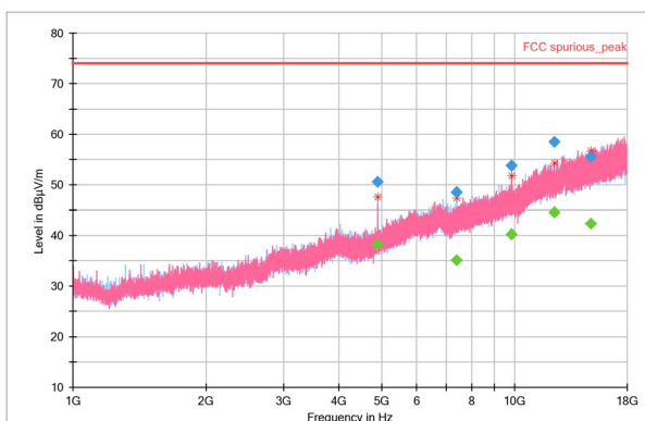
Figure 11. 1-18GHz Peak
