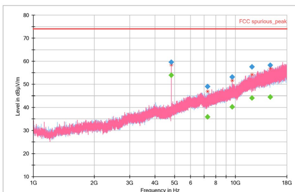
Figure 4. 1-18GHz Peak
