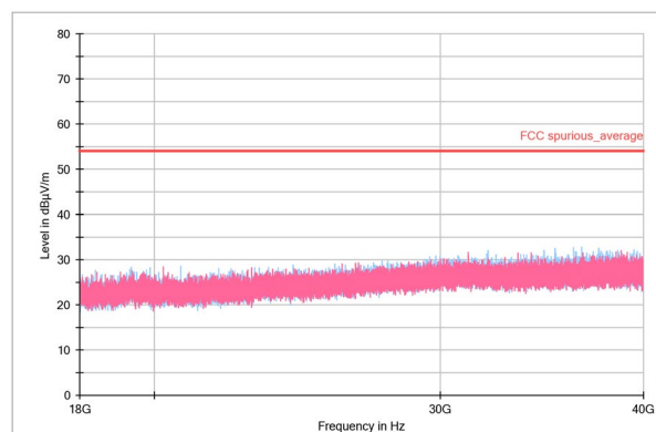
Figure 7. 18-40GHz Average
