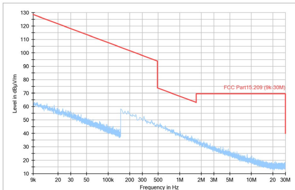
Figure 15. 9k-30MHz
