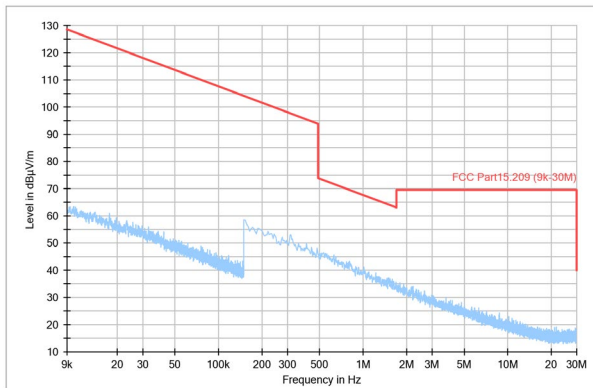
Figure 8. 9k-30MHz
