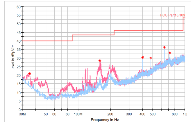
Figure 9. 30M-1GHz
