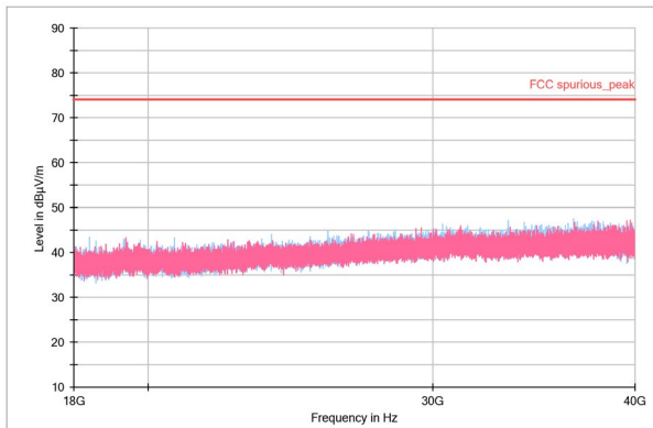
Figure 13. 18-40GHz Peak
