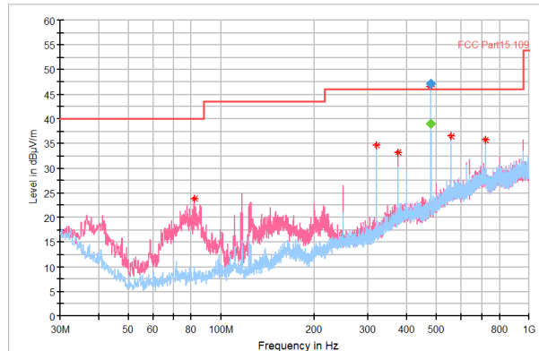
Figure 16. 30M-1GHz
