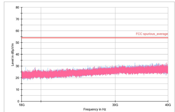
Figure 14. 18-40GHz Average
