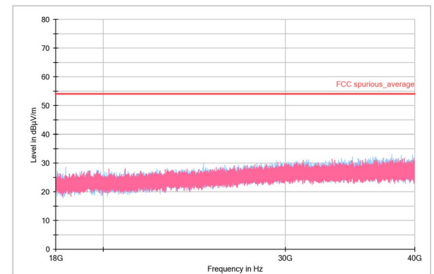
Figure 6. 18-40GHz Average
