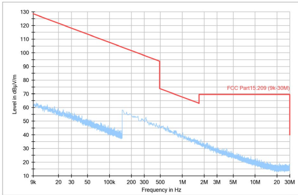
Figure 1. 9k-30MHz
