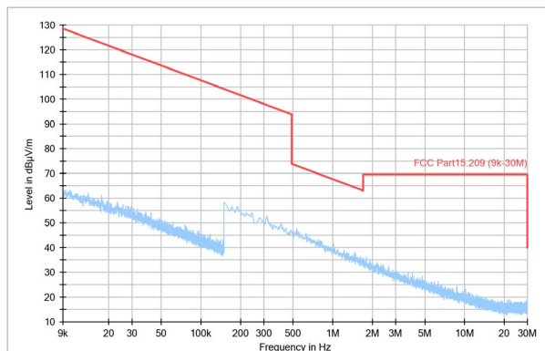
Figure 7. 9k-30MHz
