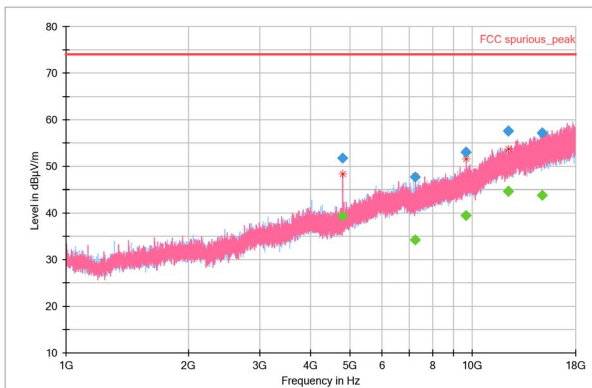
Figure 3. 1-18GHz Peak
