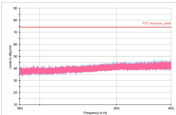
Figure 5. 18-40GHz Peak
