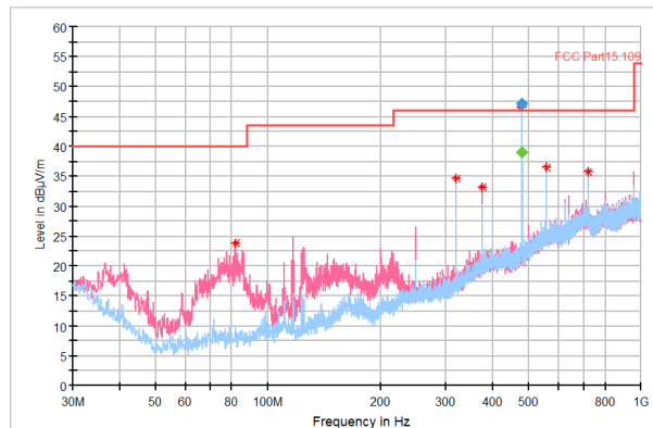
Figure 8. 30M-1GHz
