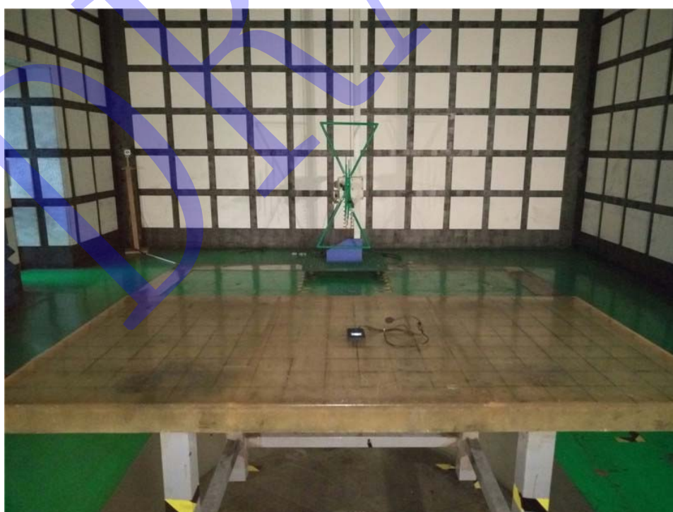
Photograph 2: Radiated Emission Test Configuration, (Below 1GHz) Back
