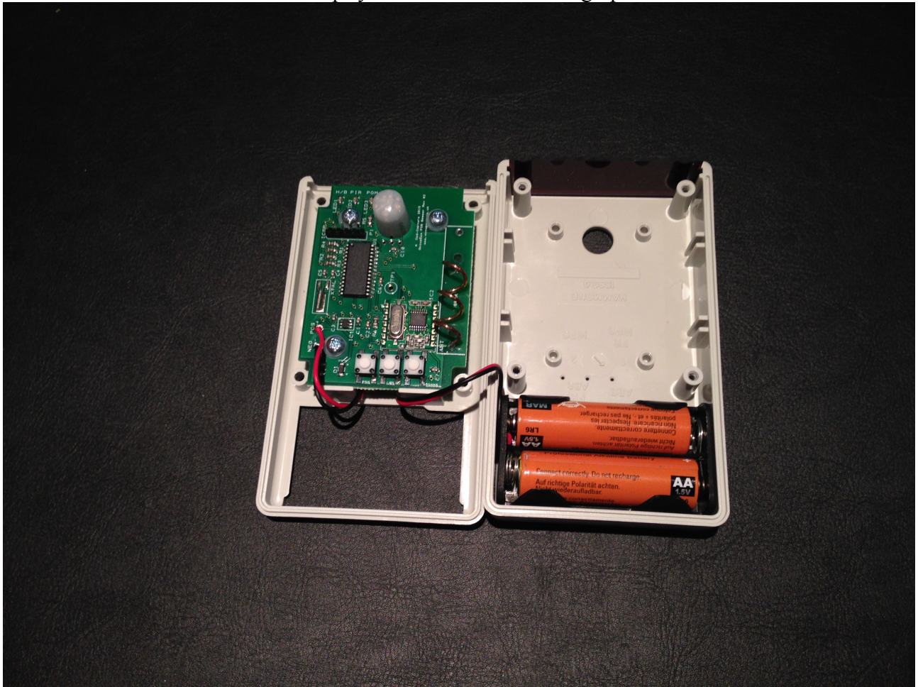
OccupEye Sensor Internal Photograph
