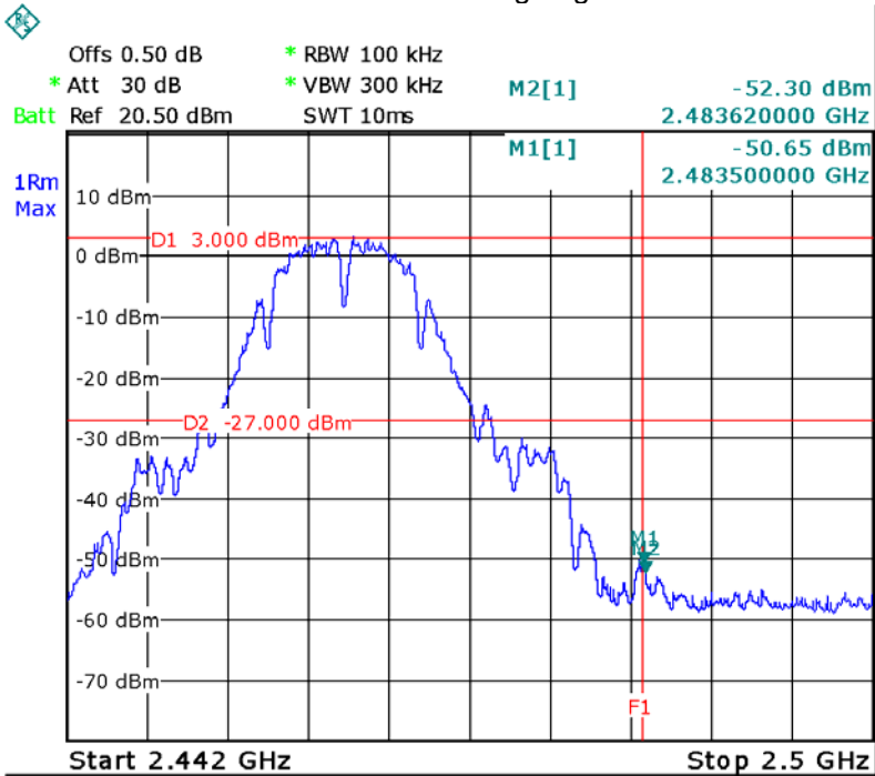
ANTA TX 11b: Band edge-right side
