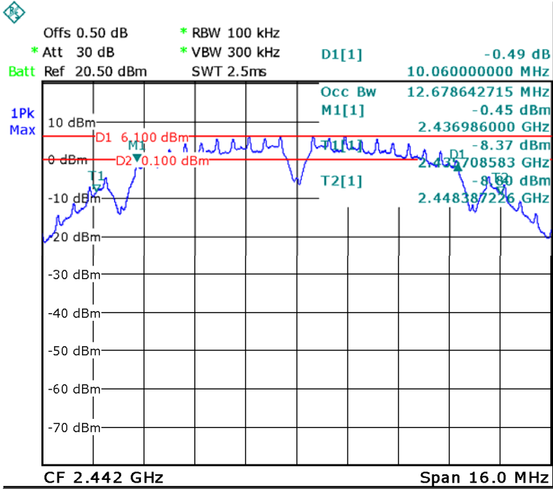
ANTB Mode: TX 11b channel 7
