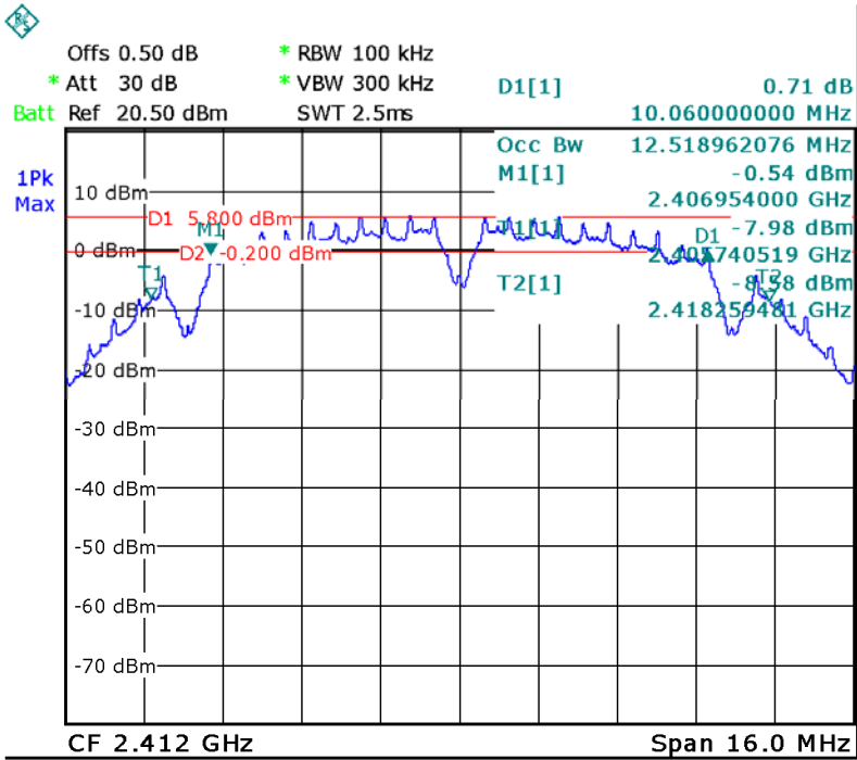
ANTB Mode: TX 11b channel 1
