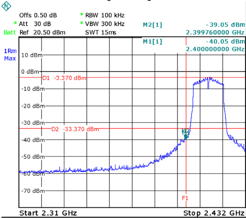
ANTA TX 11g: Band edge-left side
