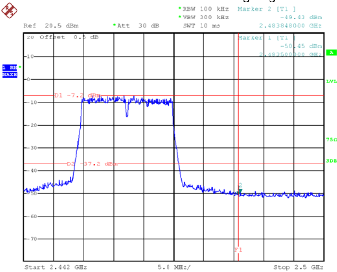
ANTB TX 11n HT20: Band edge-right side
