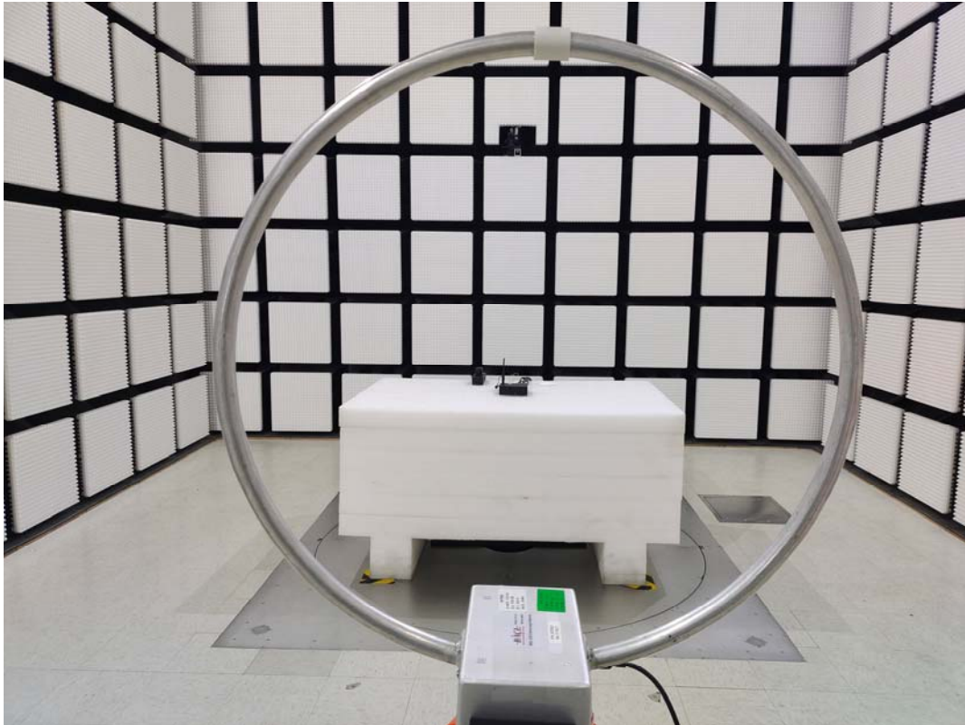
Radiated Emission 9kHz to 30MHz View Perpendicular
