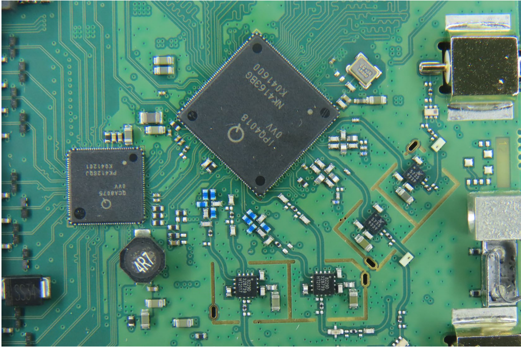
(28) EUT Photo
