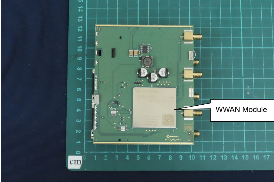
(22) EUT Photo
