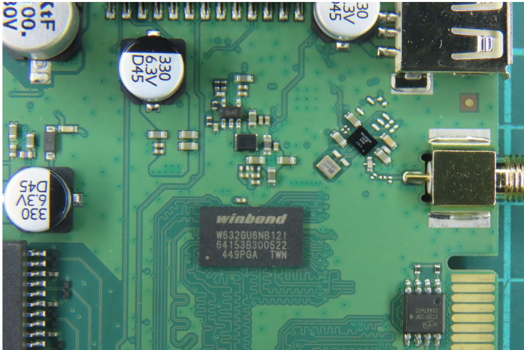
(29) EUT Photo
