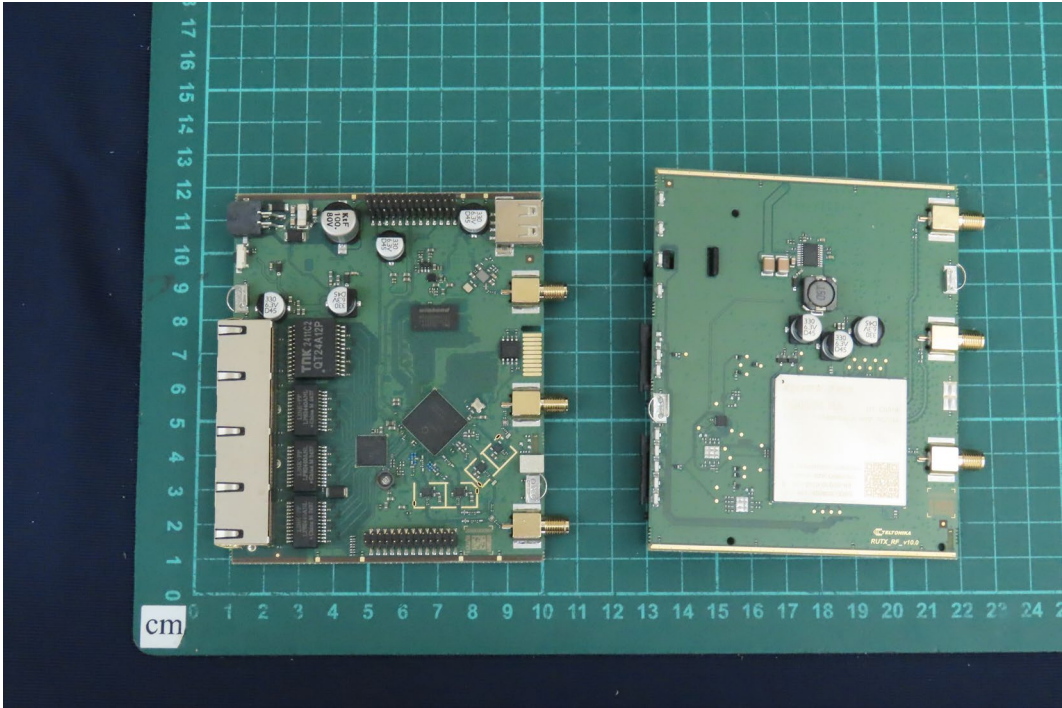
(23) EUT Photo
