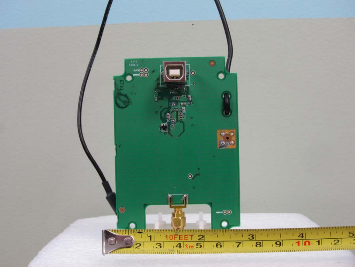
Transceiver Board Rear
