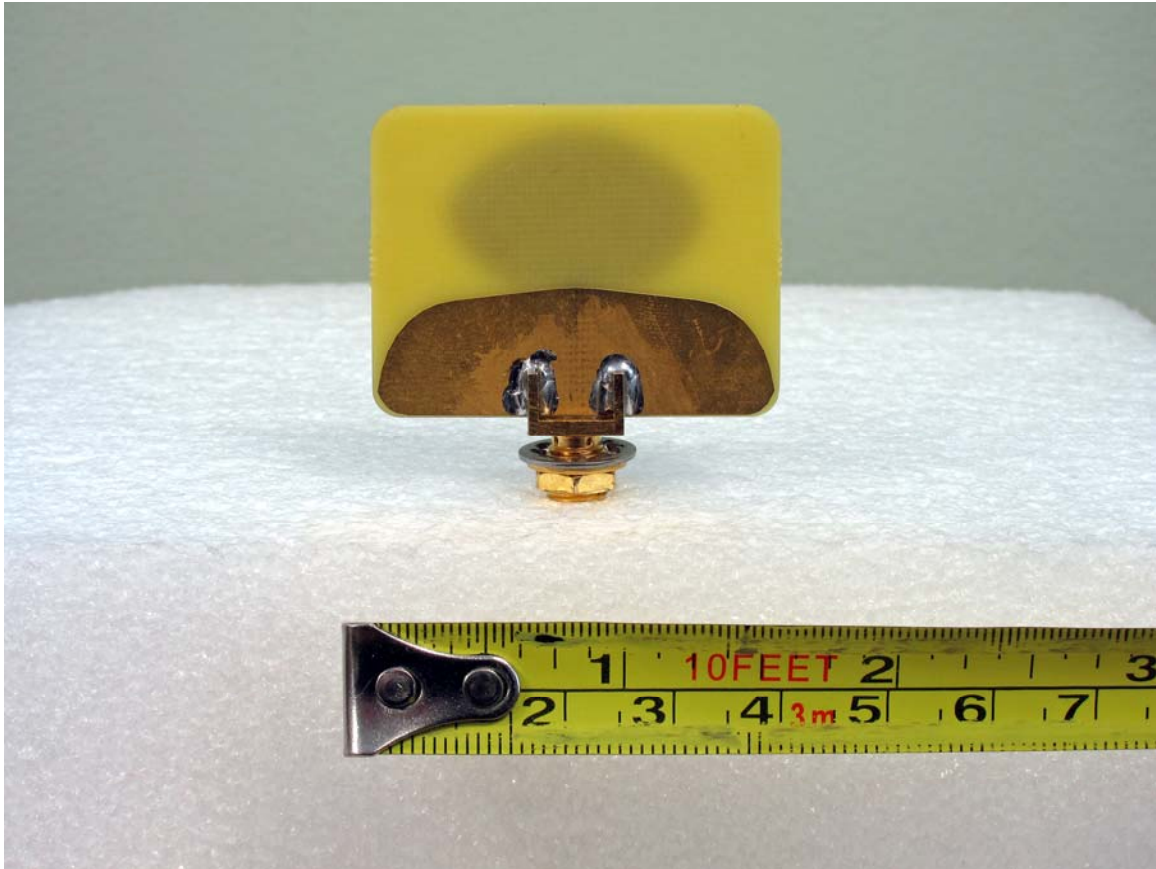
Transmit Antenna Section –Antenna rear
