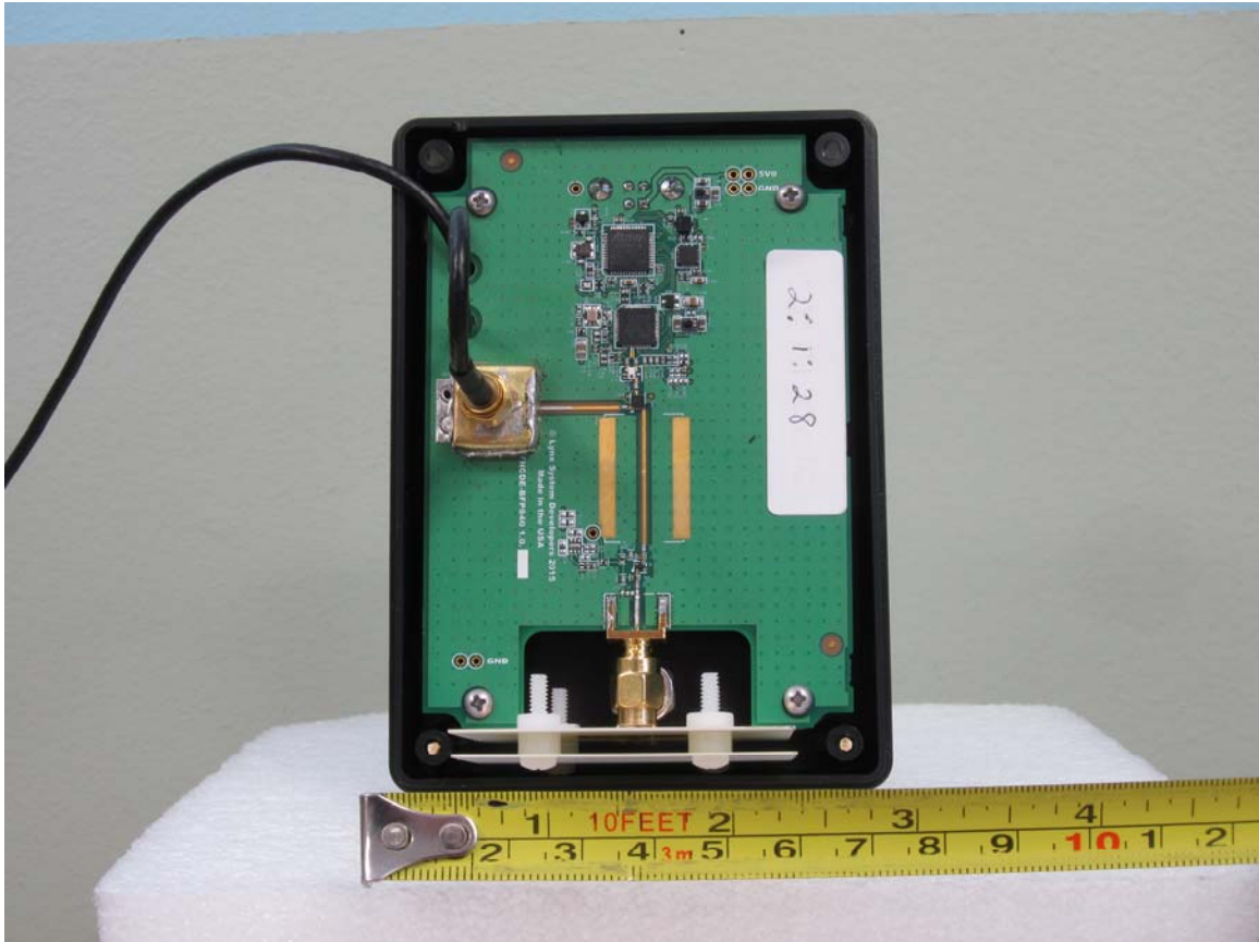
Transceiver Section Cover Off
