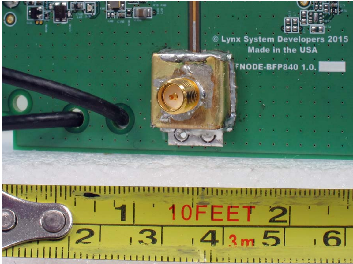
Transceiver Board – Front Connector Profile
