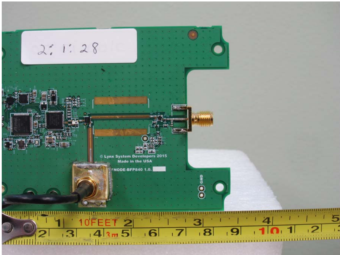
Transceiver Board Close up
