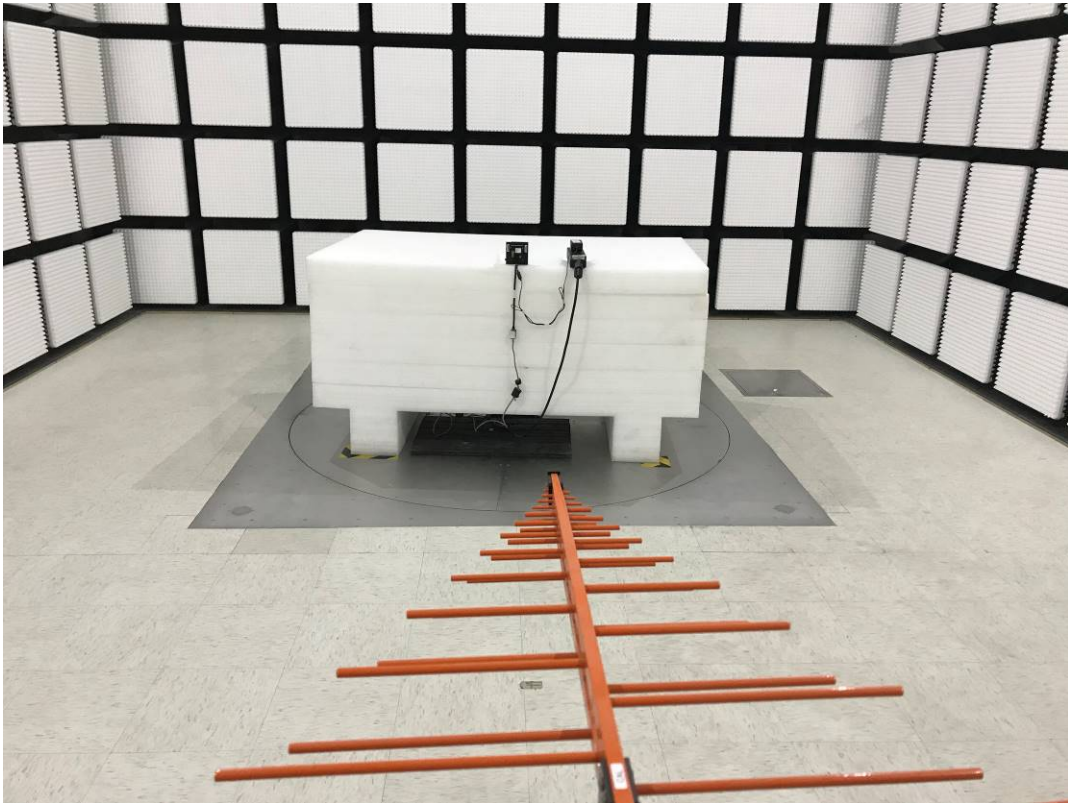
Radiated Emissions Below 1G rear View – Adapter
