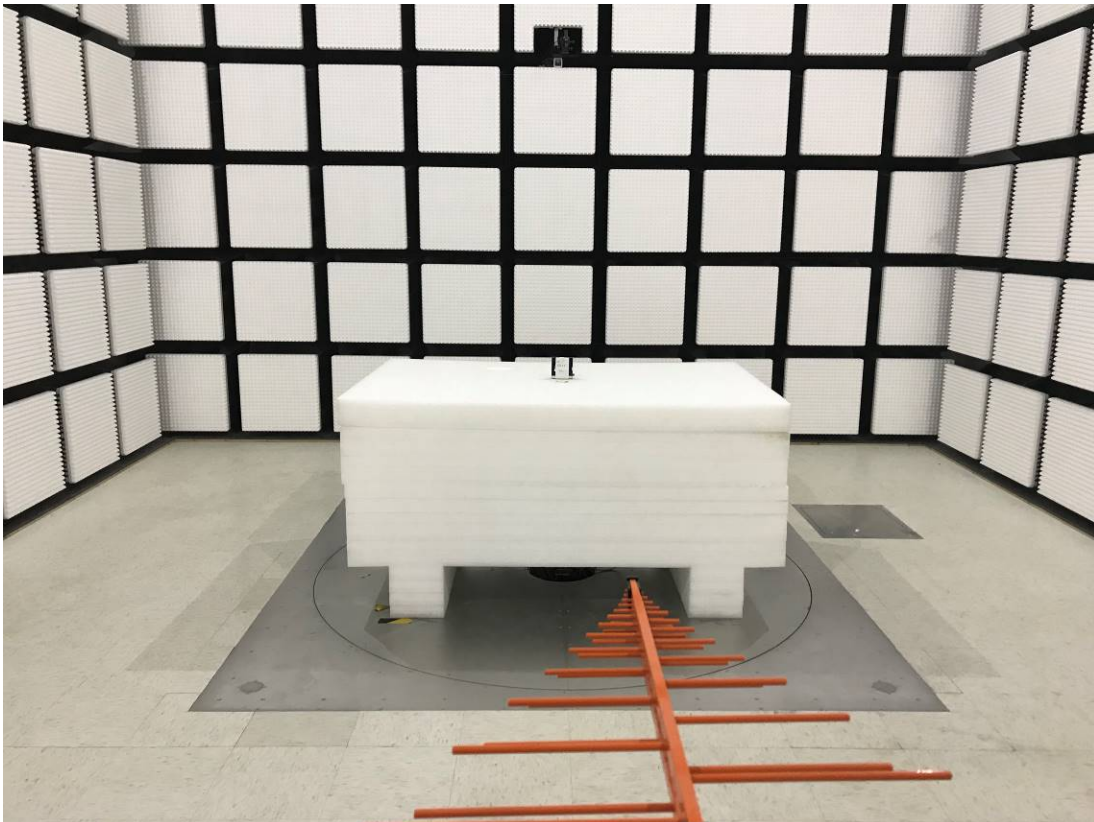
Radiated Emission 30MHz-1GHz View PoE
