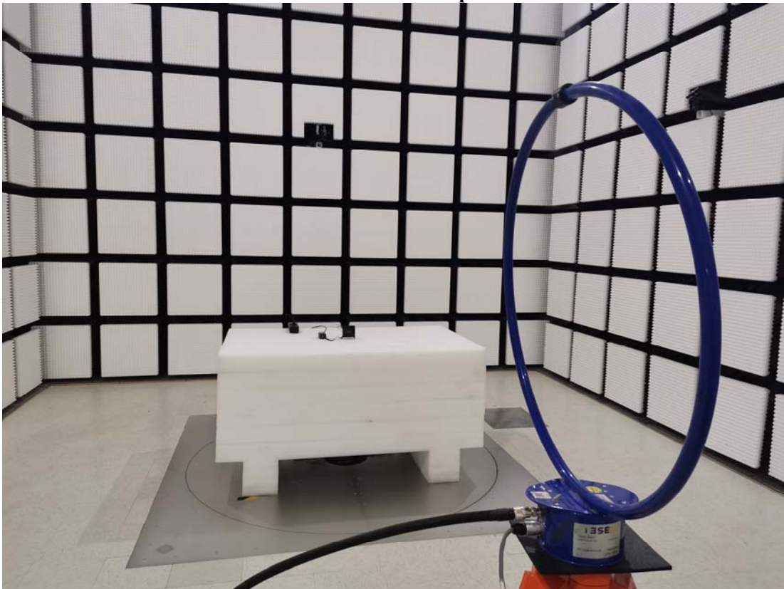
Radiated Emission 9kHz-30MHz Perpendicular View POE
