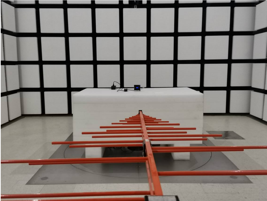
Radiated Emission Below 1GHz View Adapter
