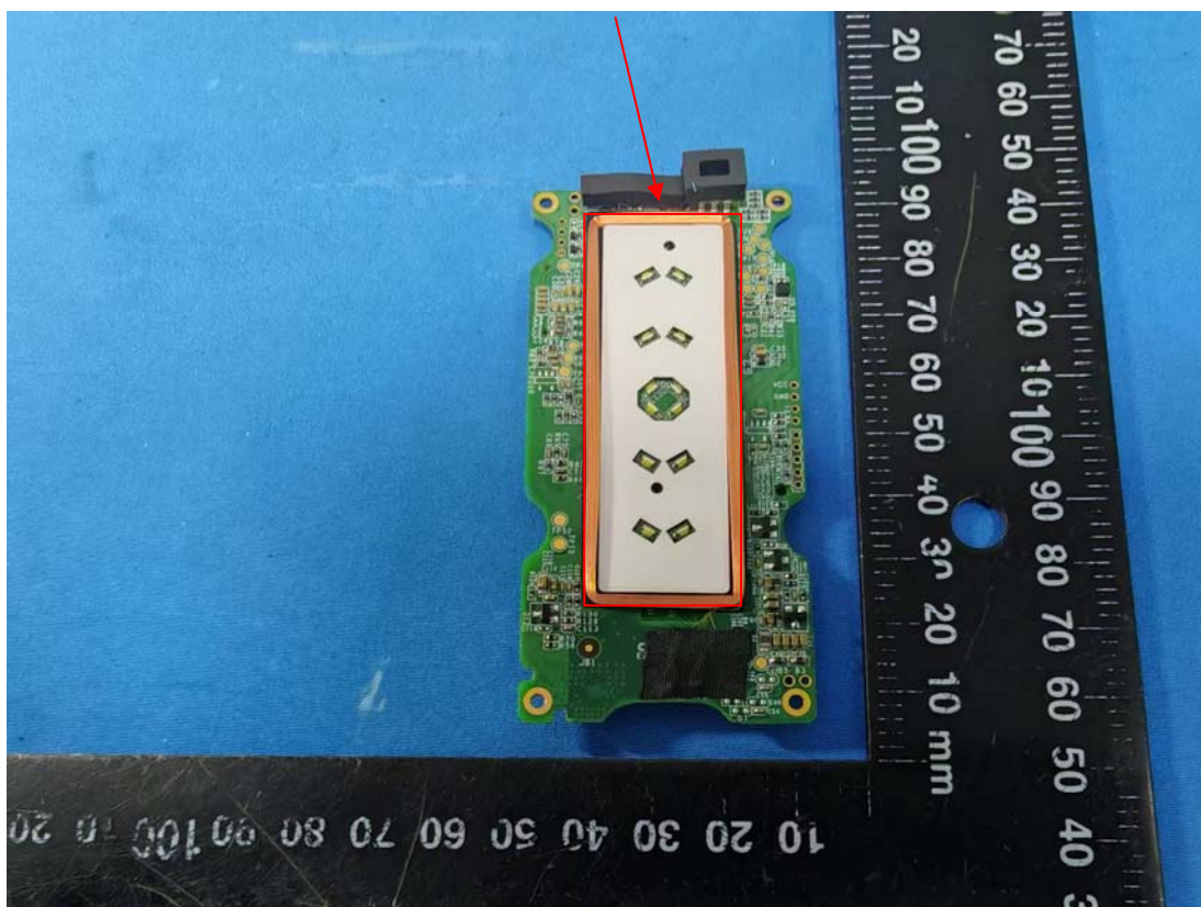
RFID(125k) Antenna
