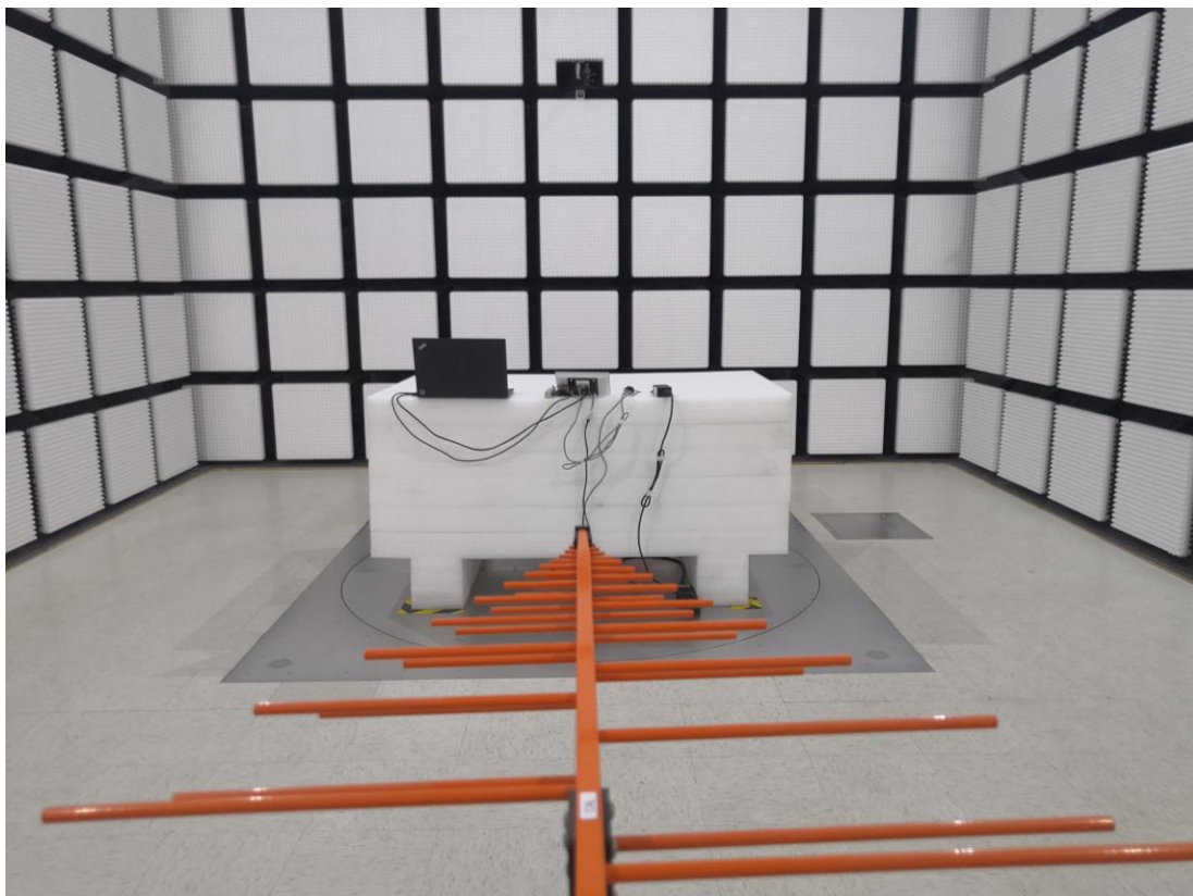
Radiated Emission Below 1G View POE
