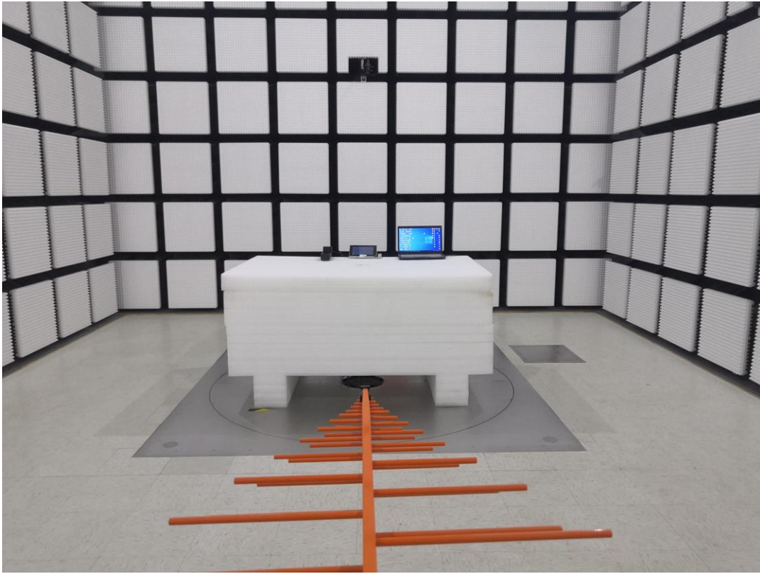
Radiated Emission Below 1G View Adapter
