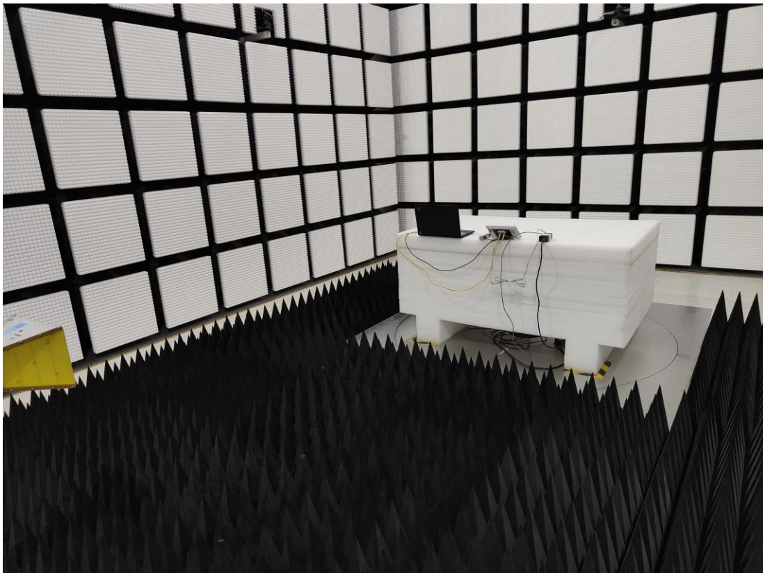
Radiated Emission Above 1G View POE
