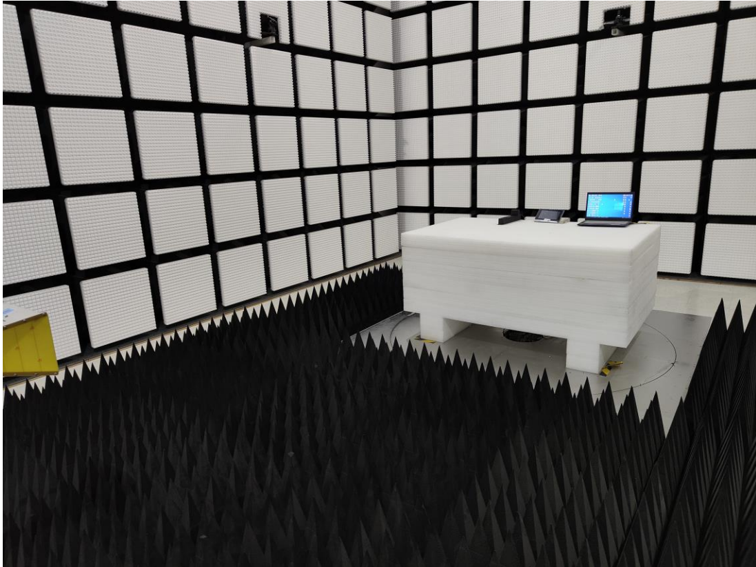
Radiated Emission Above 1G View Adapter
