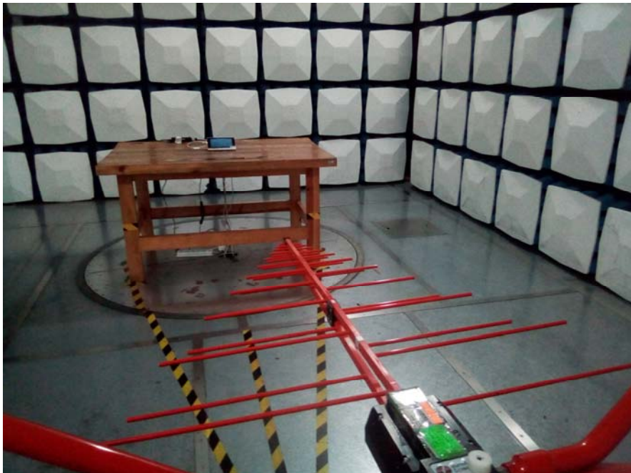
POE Radiated Emission View (Below 1GHz)
