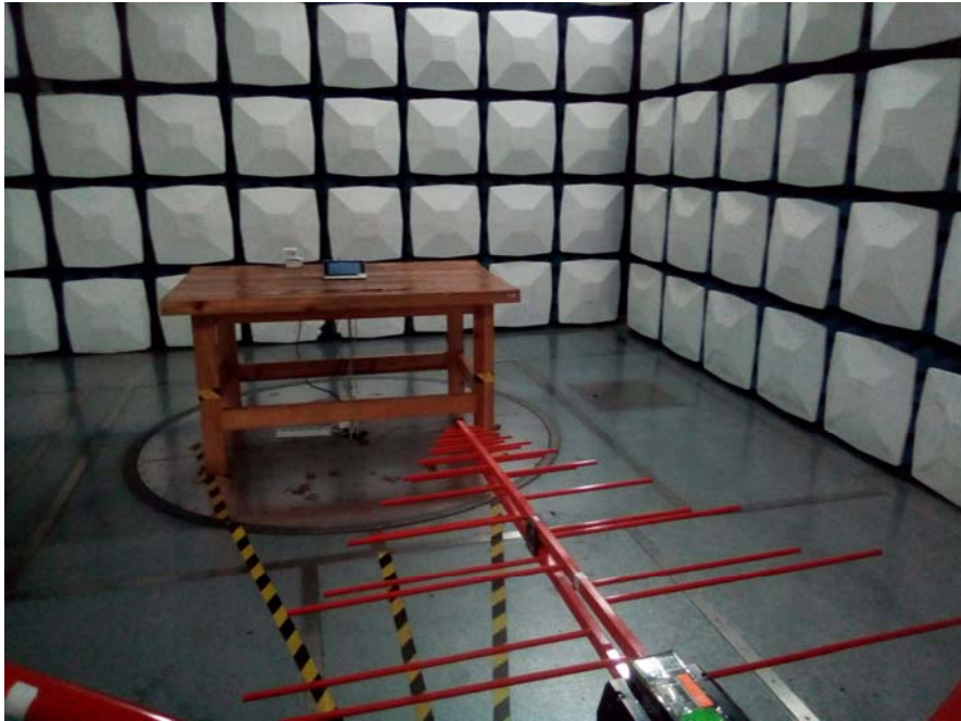
Adapter Radiated Emission View (Below 1GHz)
