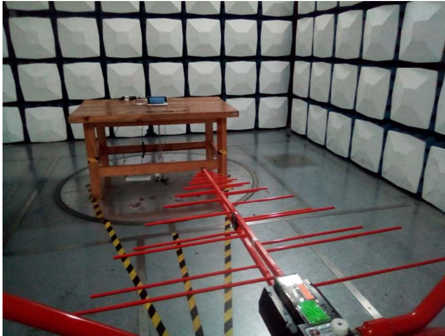
POE Radiated Emission Below 1GHz View
