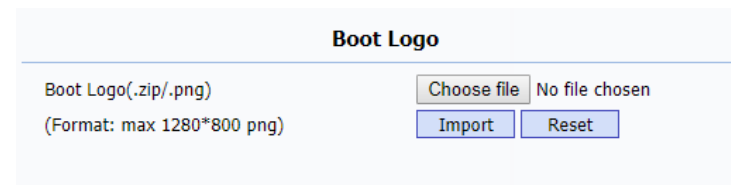
Figure 3.4.10 -1 Boot logo
