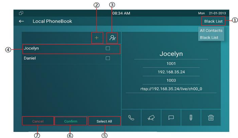
Figure3.5.4-1 Black list
