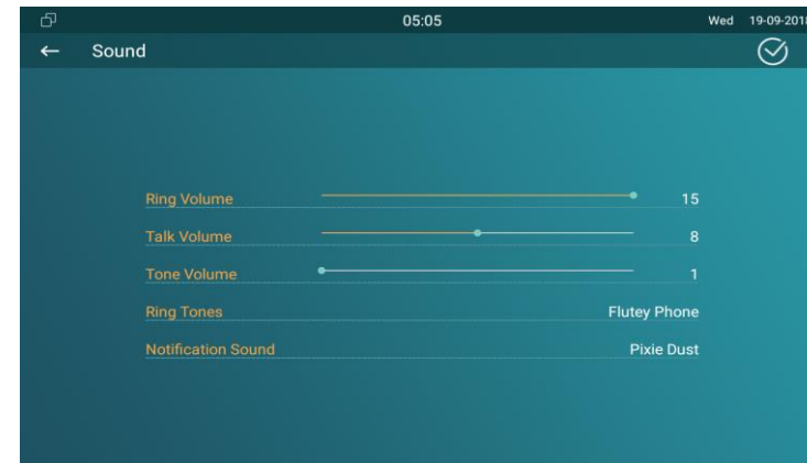
Figure 3.4.6 -1 Sound setting
