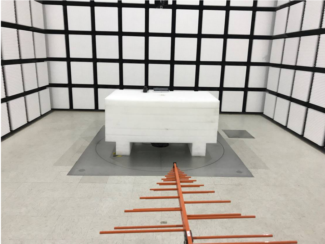
Radiated Emissions Below 1G rear View –AC/DC Adapter
