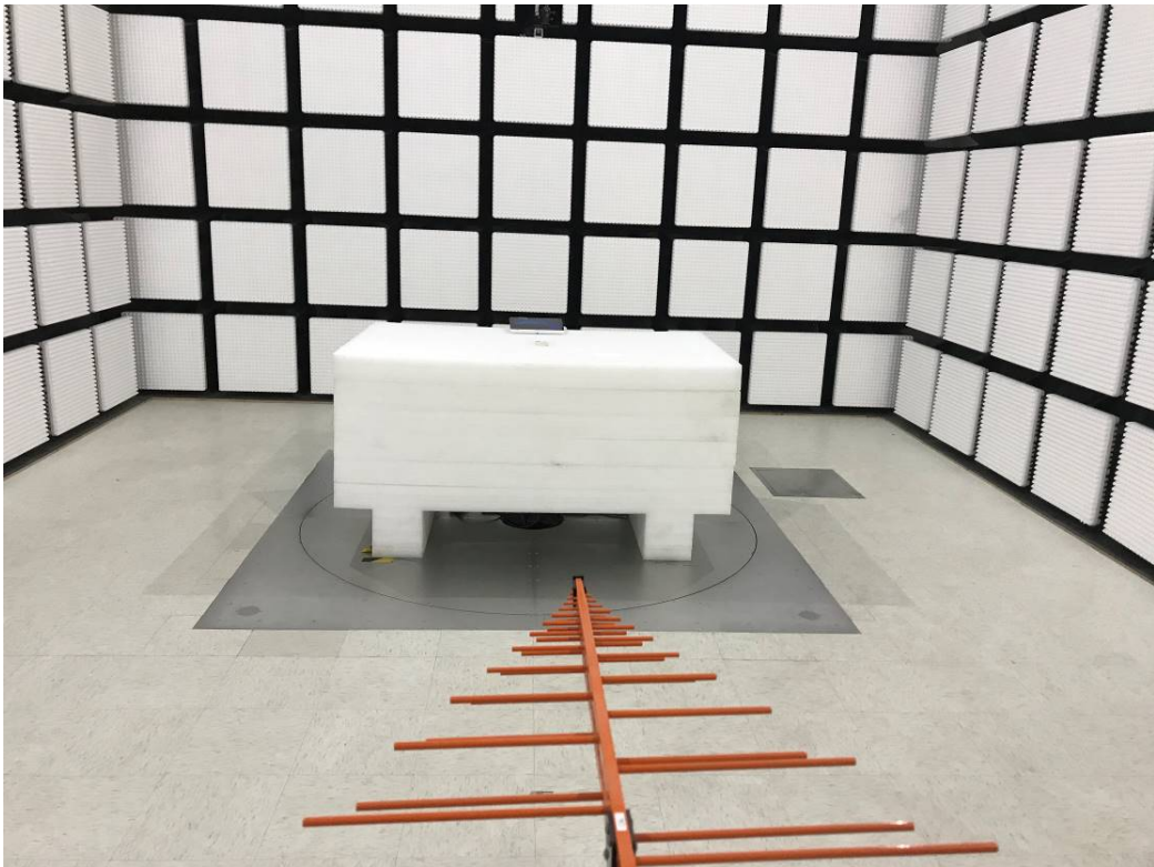
Radiated Emissions Below 1G rear View –PoE Adapter
