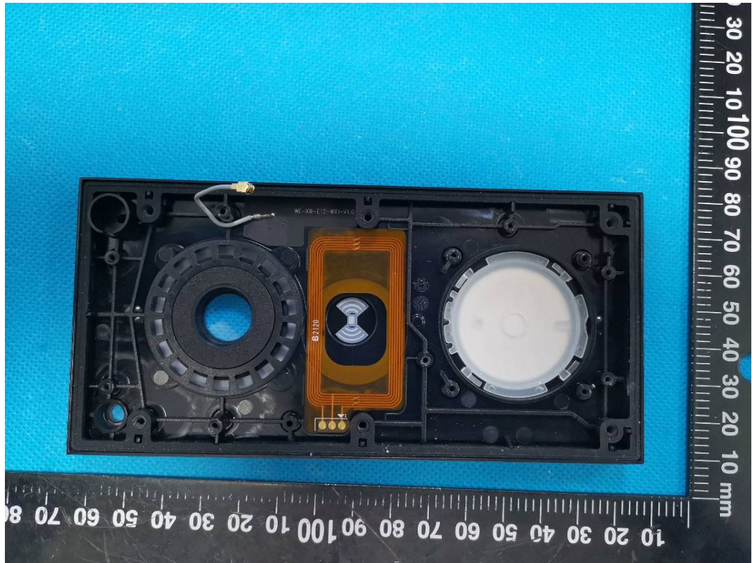
WiFi Antenna
