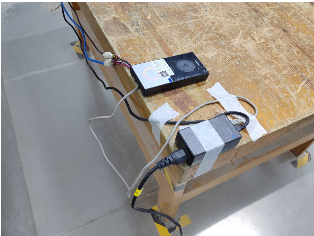
Conducted Emissions Side View- POE
