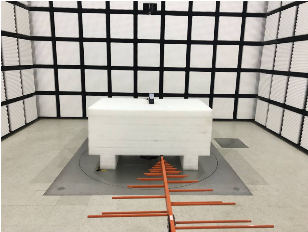
Radiated Emissions Below 1G View -POE
