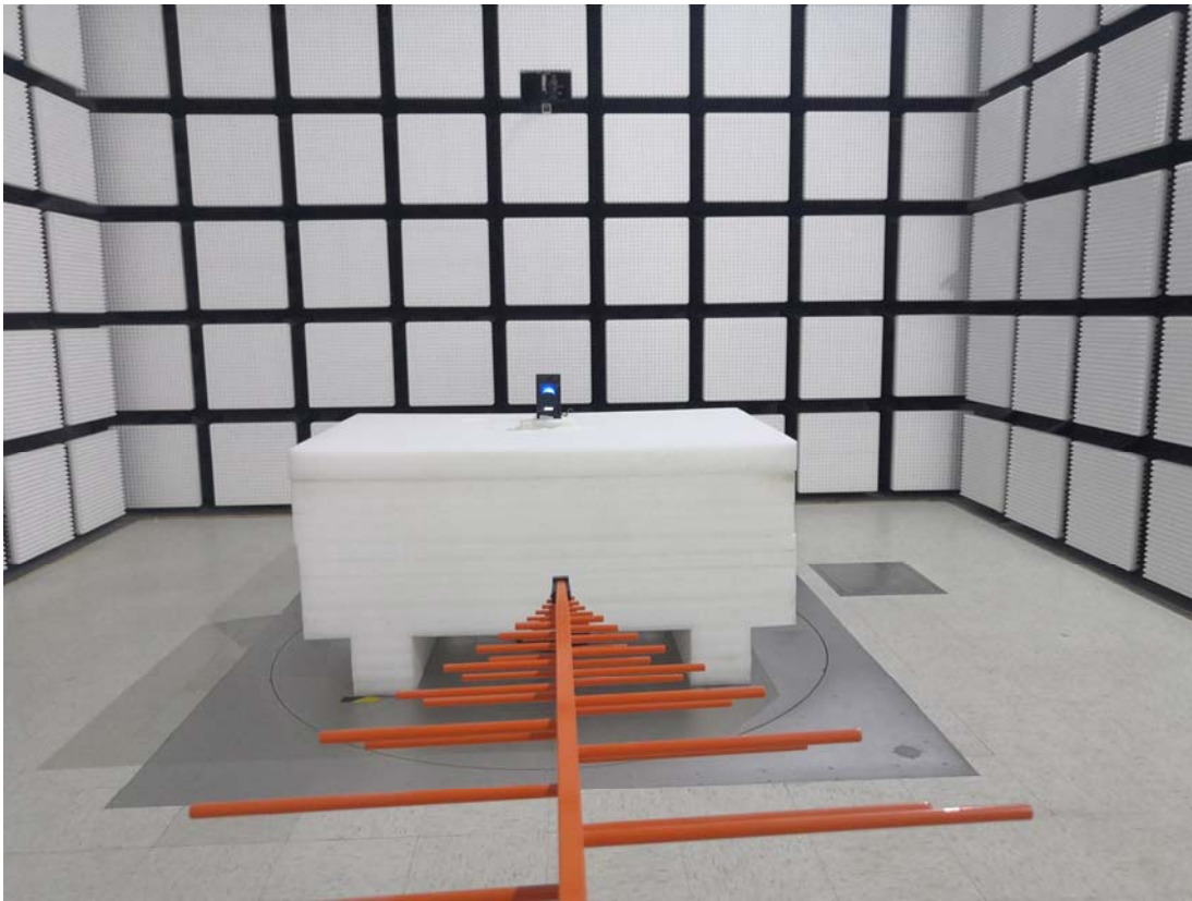
Radiated Emission Below 1GHz Adapter- A05C
