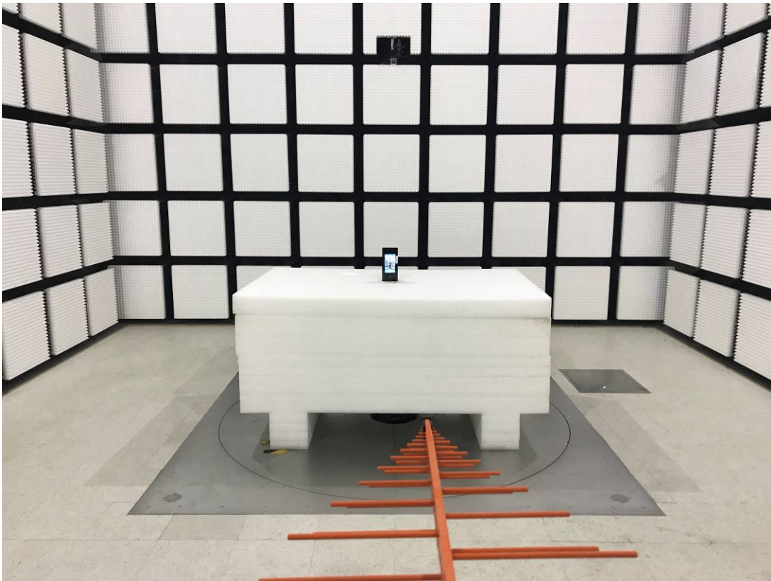
Radiated Emission Below 1GHz Adapter- E16C
