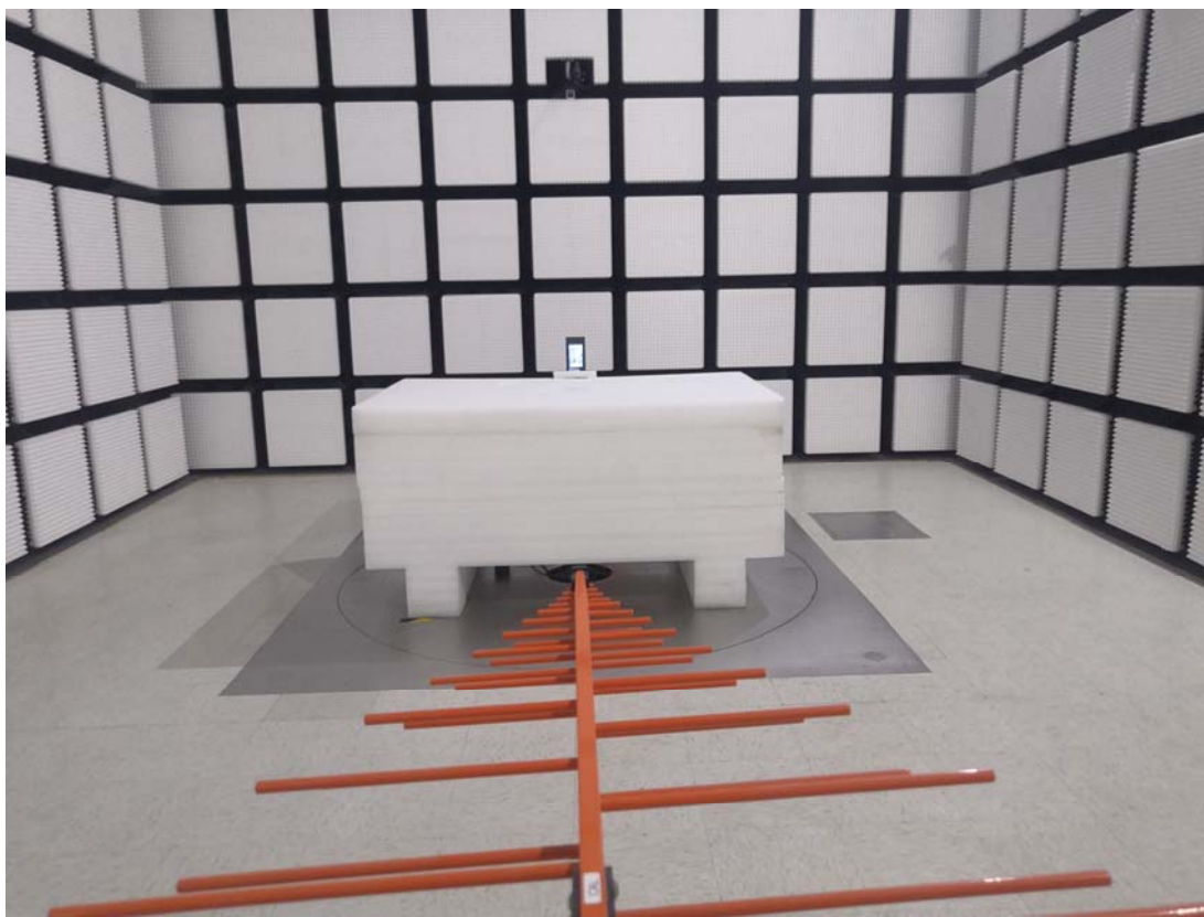
Radiated Emission Below 1G rear View POE- A05C
