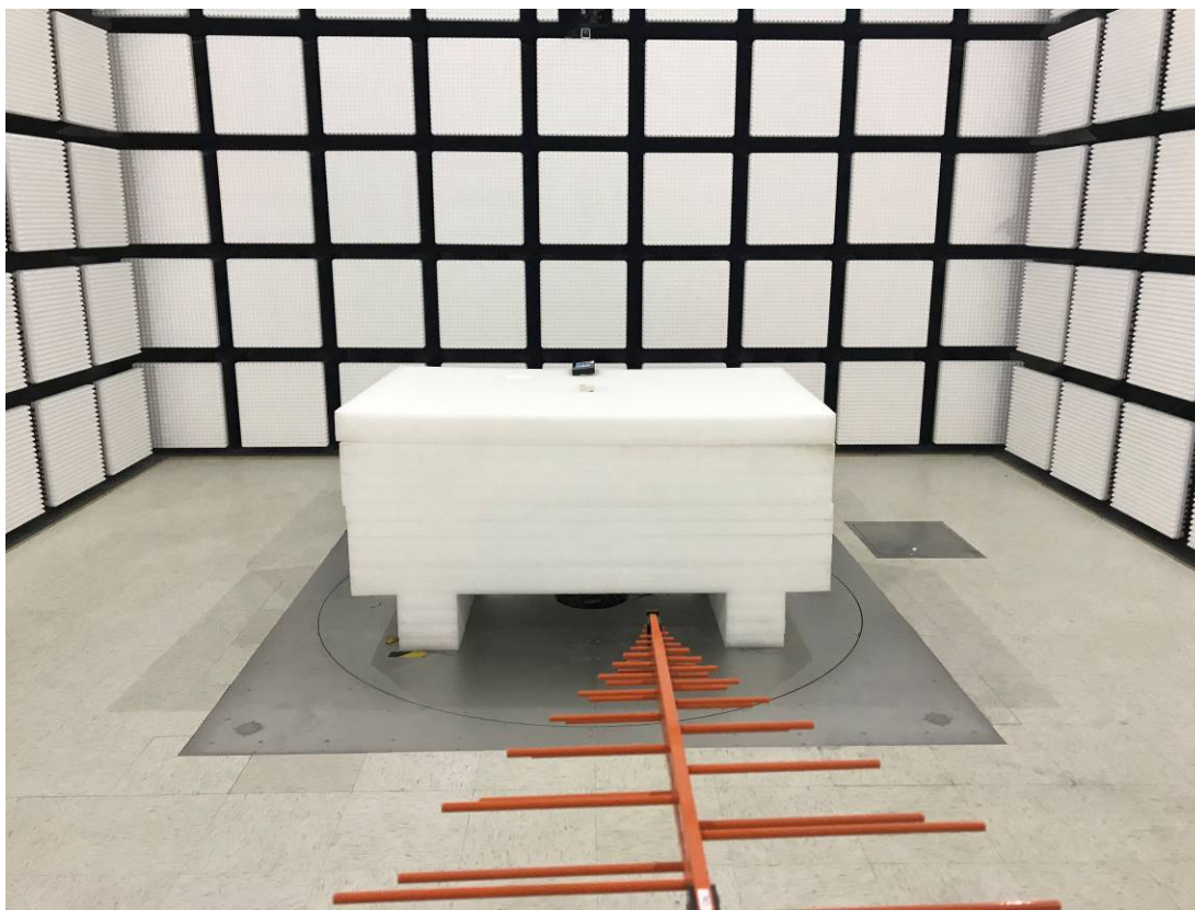
Radiated Emission Below 1G rear View POE- E16C
