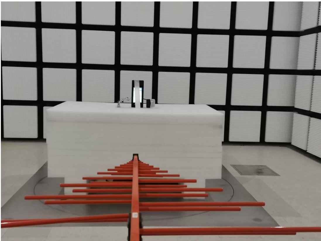
Radiated Emission Below 1GHz View POE
