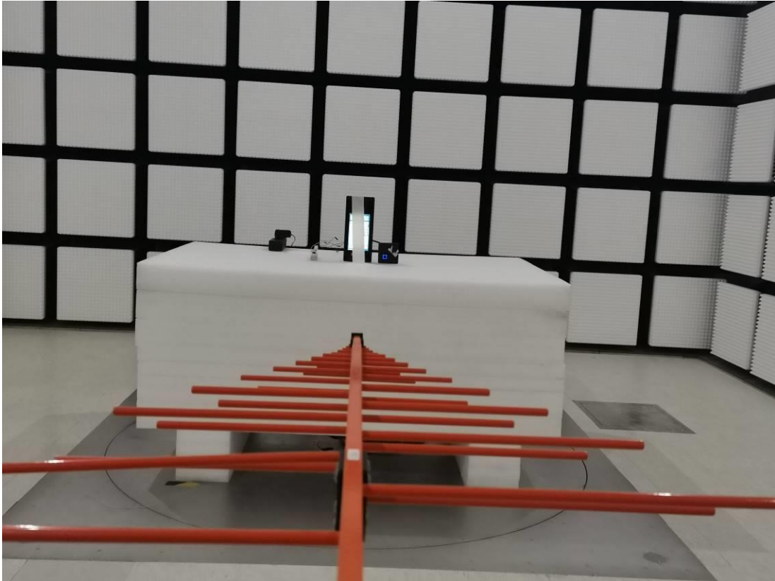
Radiated Emission Above 1GHz View Adapter
