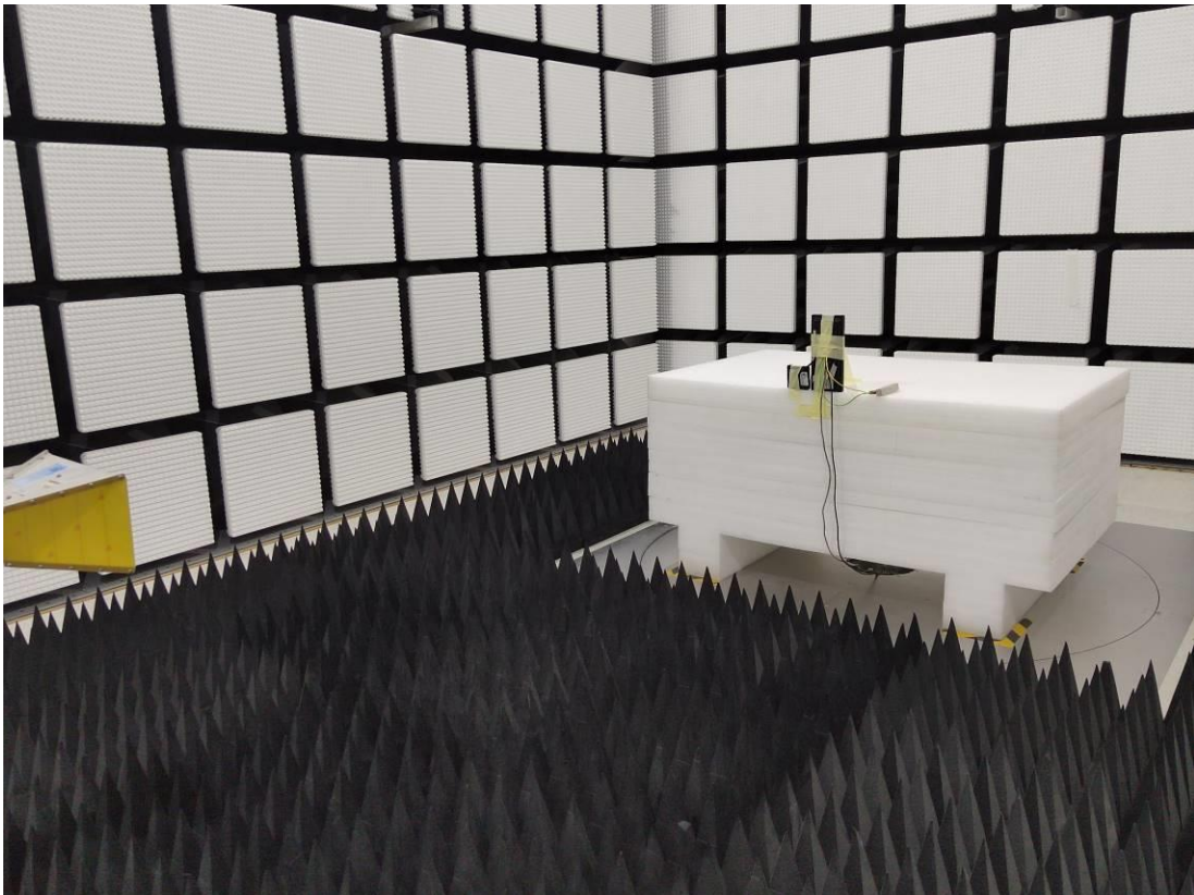
Radiated Emission Above 1G rear View POE
