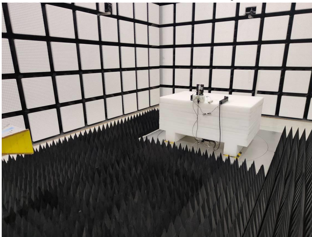
Radiated Emission Above 1G rear View Adapter
