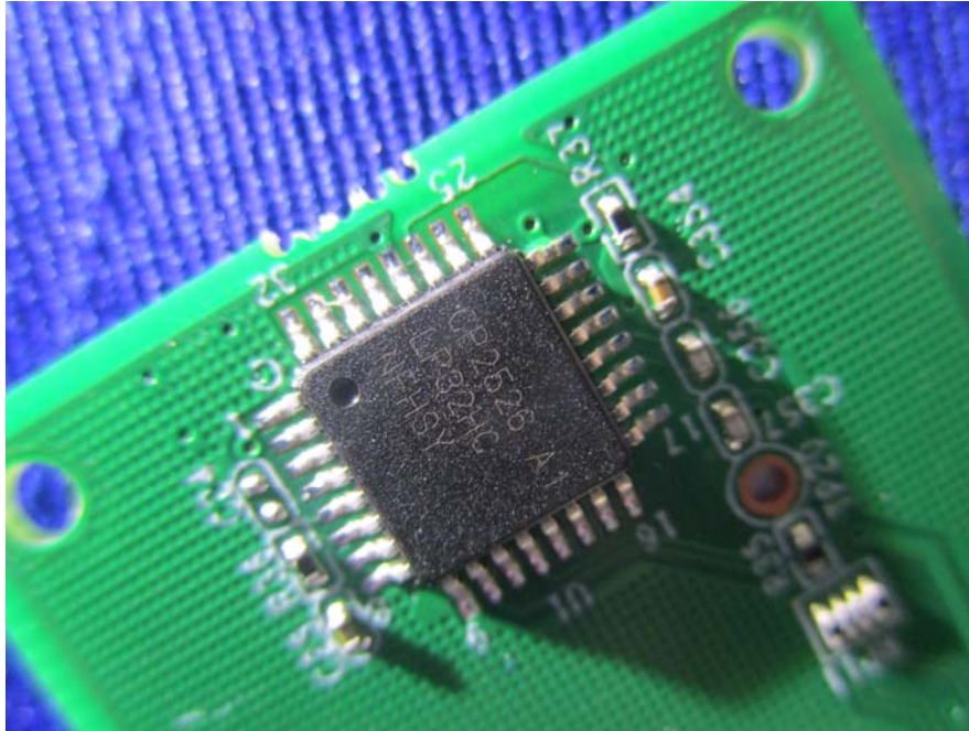
EUT – Touch Screen Board Chip View
