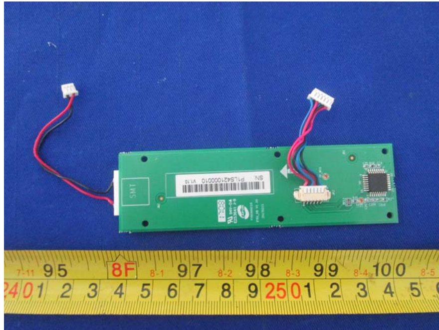
EUT – Touch Screen Board Top View
