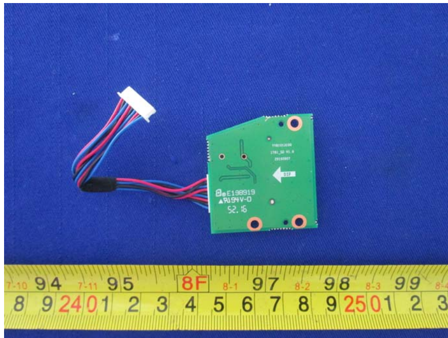
EUT – Memory Card Board Bottom View
