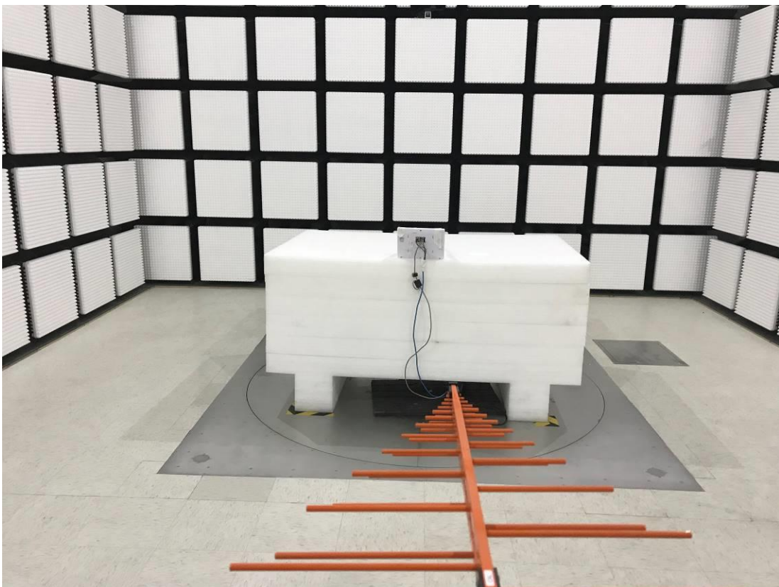
Radiated Emission Below 1G View POE
