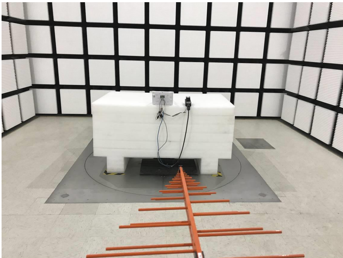
Radiated Emission Below 1G View Adapter
