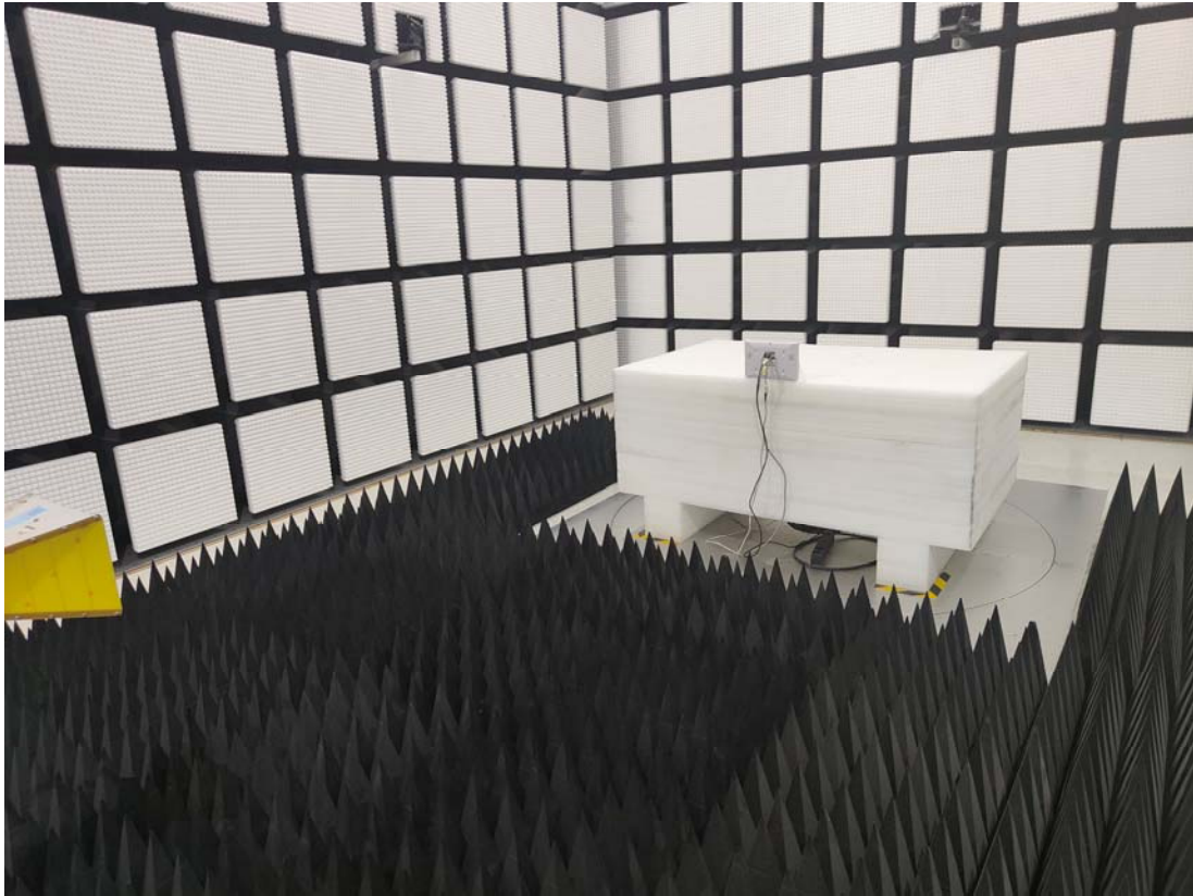
Radiated Emission Above 1G rear View- POE Adapter
