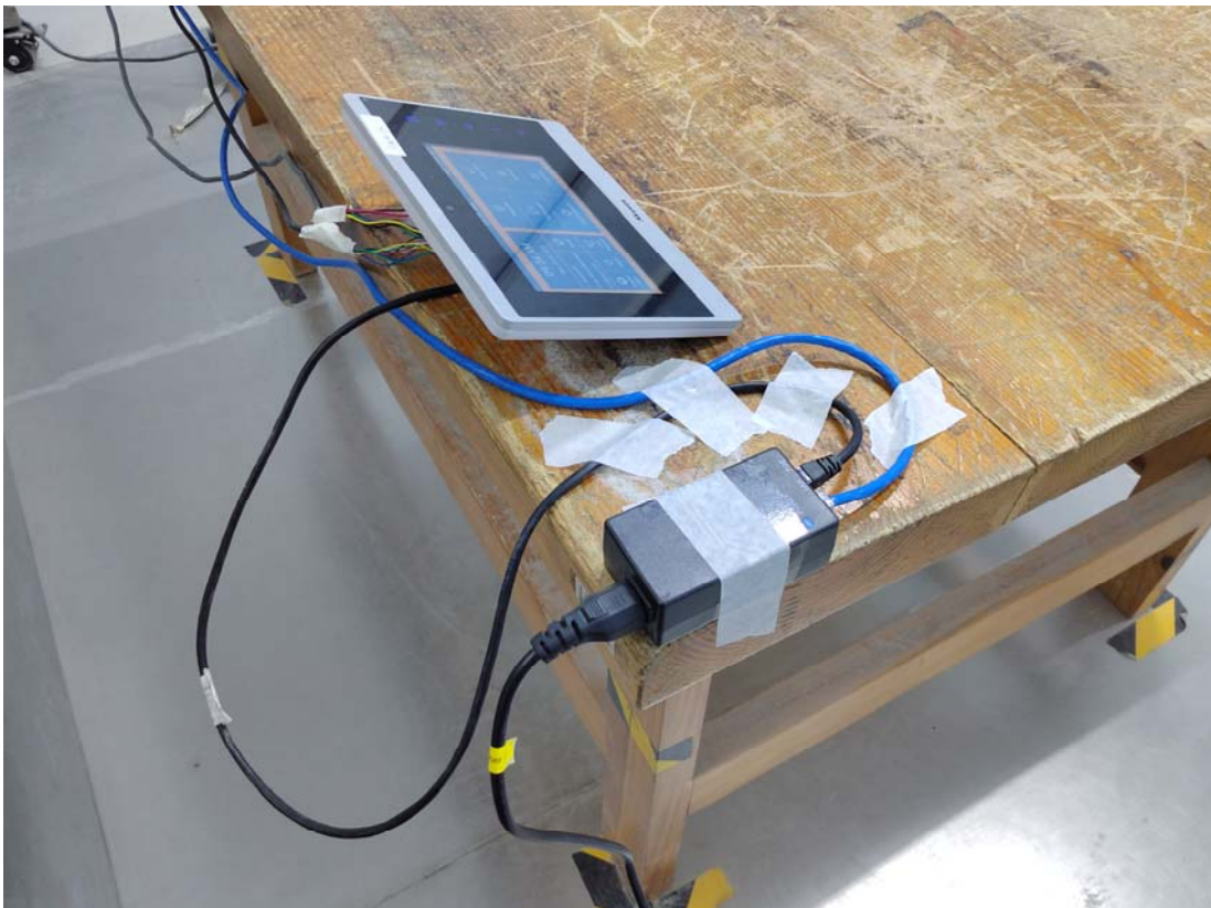
Conducted Emissions Side View- POE Adapter
