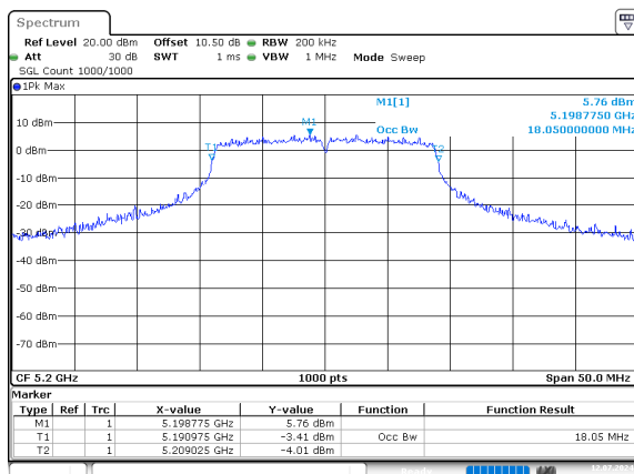
n20_5200MHz_Chain 0 1
