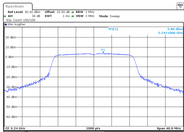
n20_5240MHz_Chain 0
