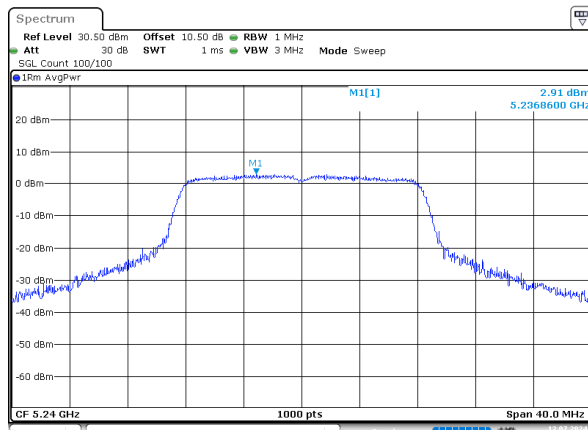
a_5240MHz_Chain 0
