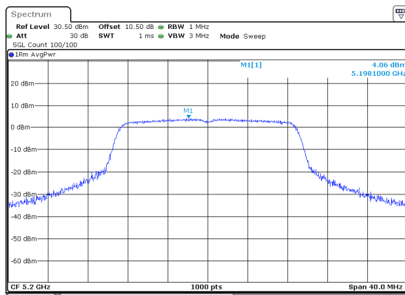
n20_5200MHz_Chain 0
