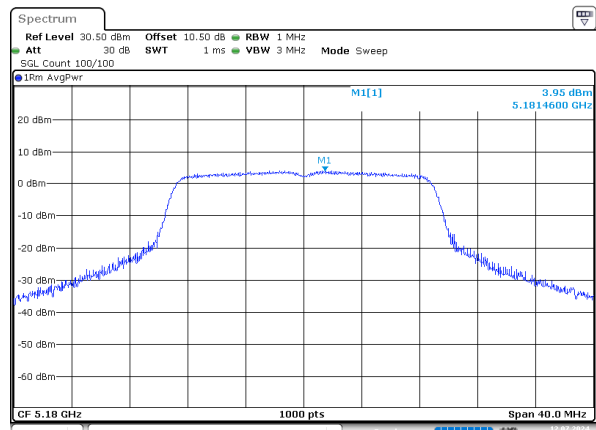
n20_5180MHz_Chain 0
