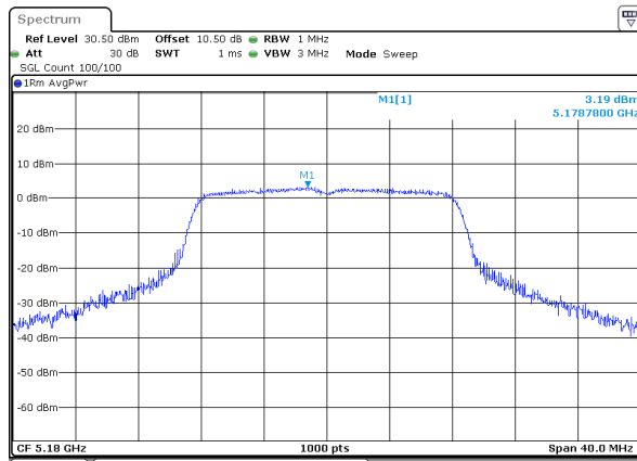
a_5180MHz_Chain 0
