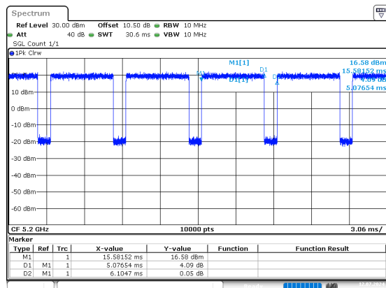
n20_5200MHz_Chain 0
