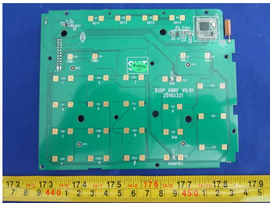
EUT – Keyboard Shilding Off View
