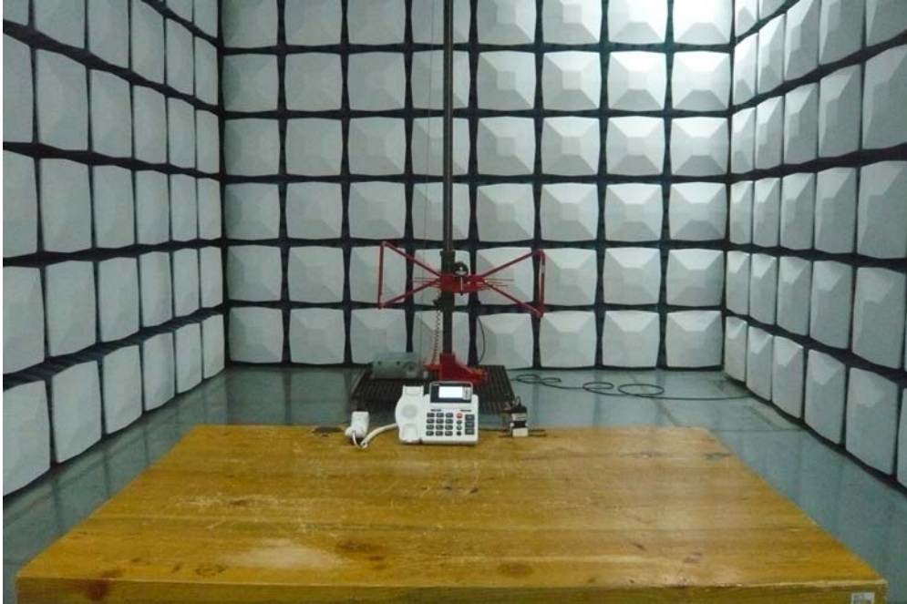
Radiated Emissions –Front View (Adapter)
