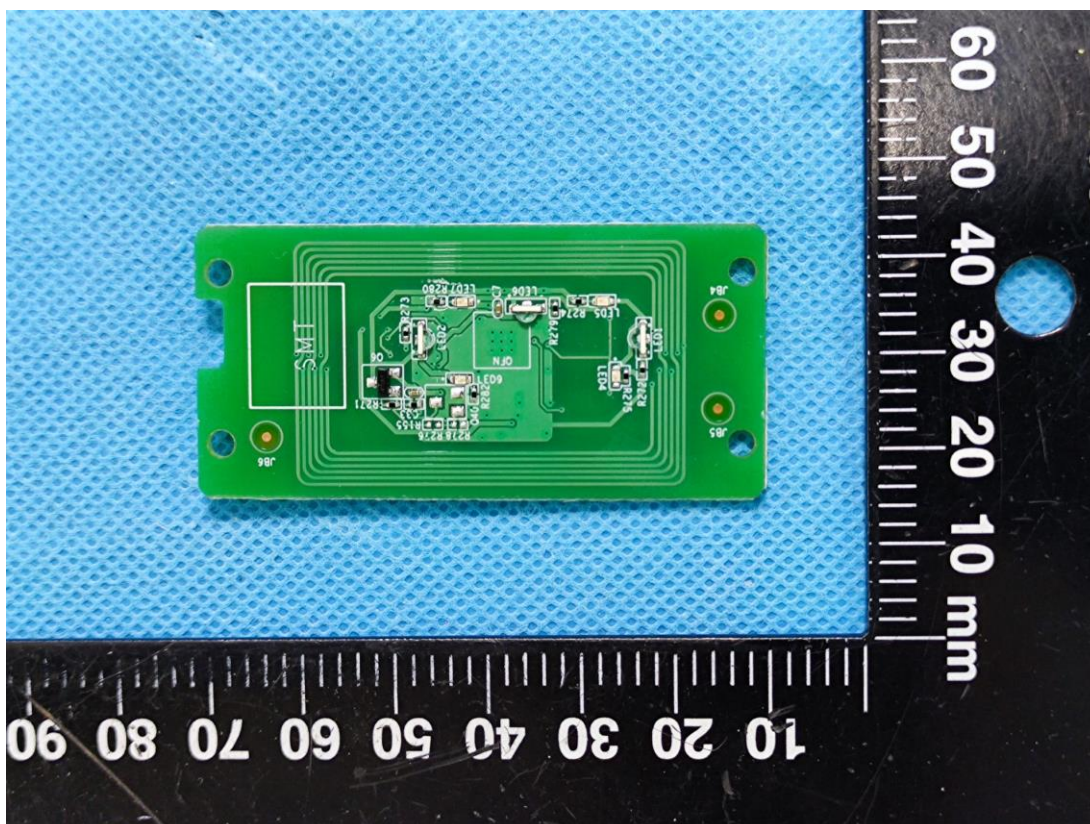
13.56MHz Antenna
