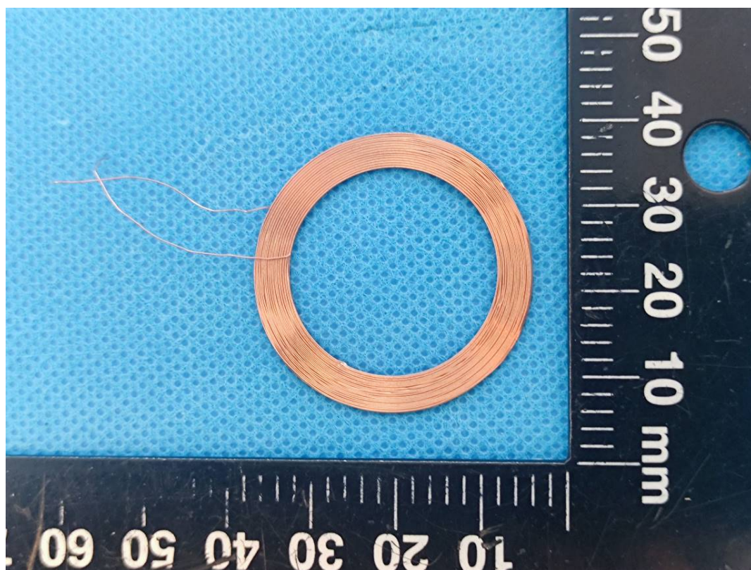
125k antenna
