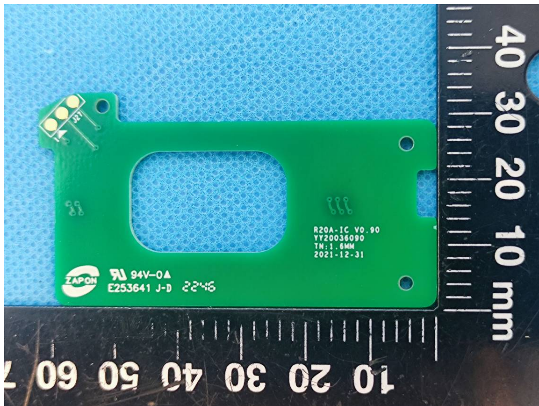
125k antenna
