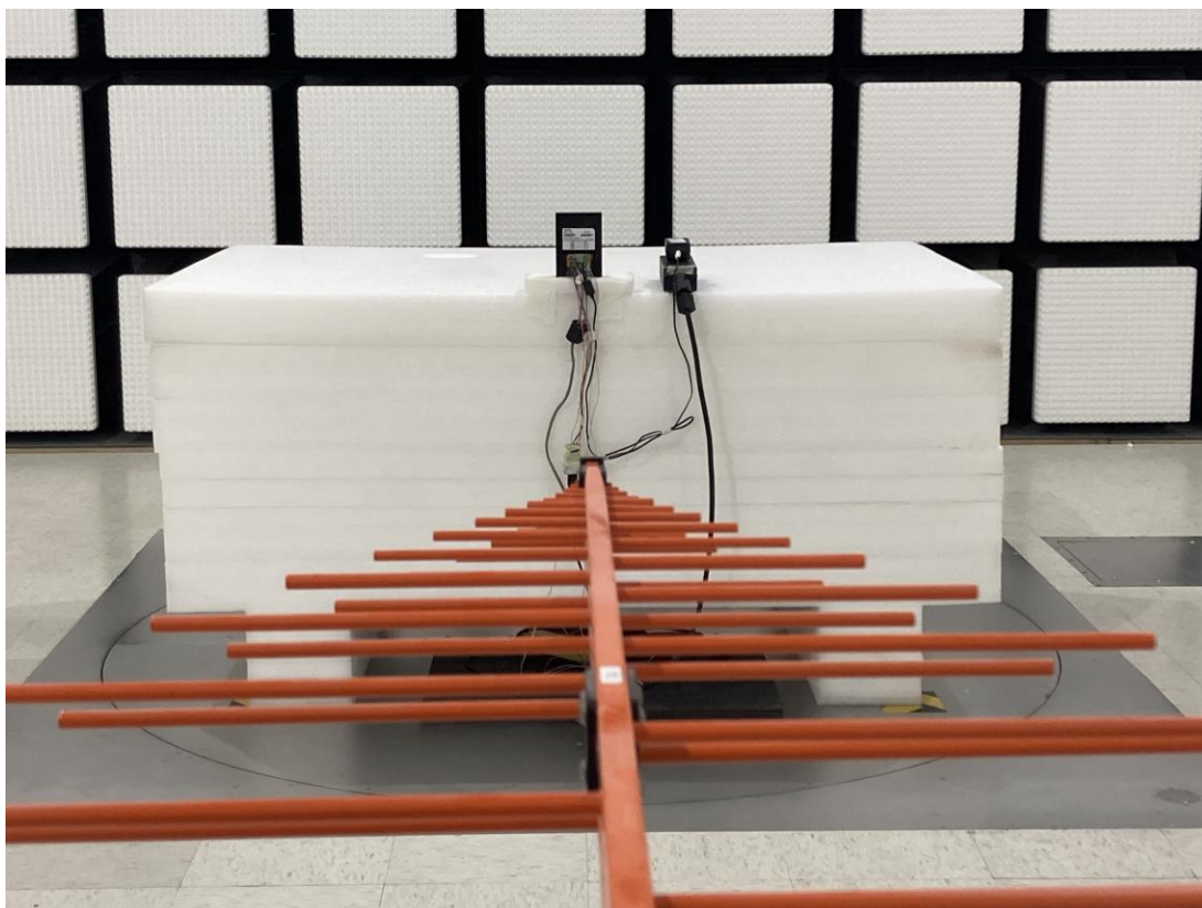
Radiated Emission Below 1G rear View -M1
