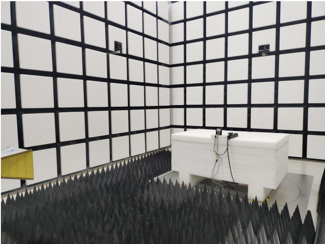
Radiated Emission Above 1G rear View -M1
