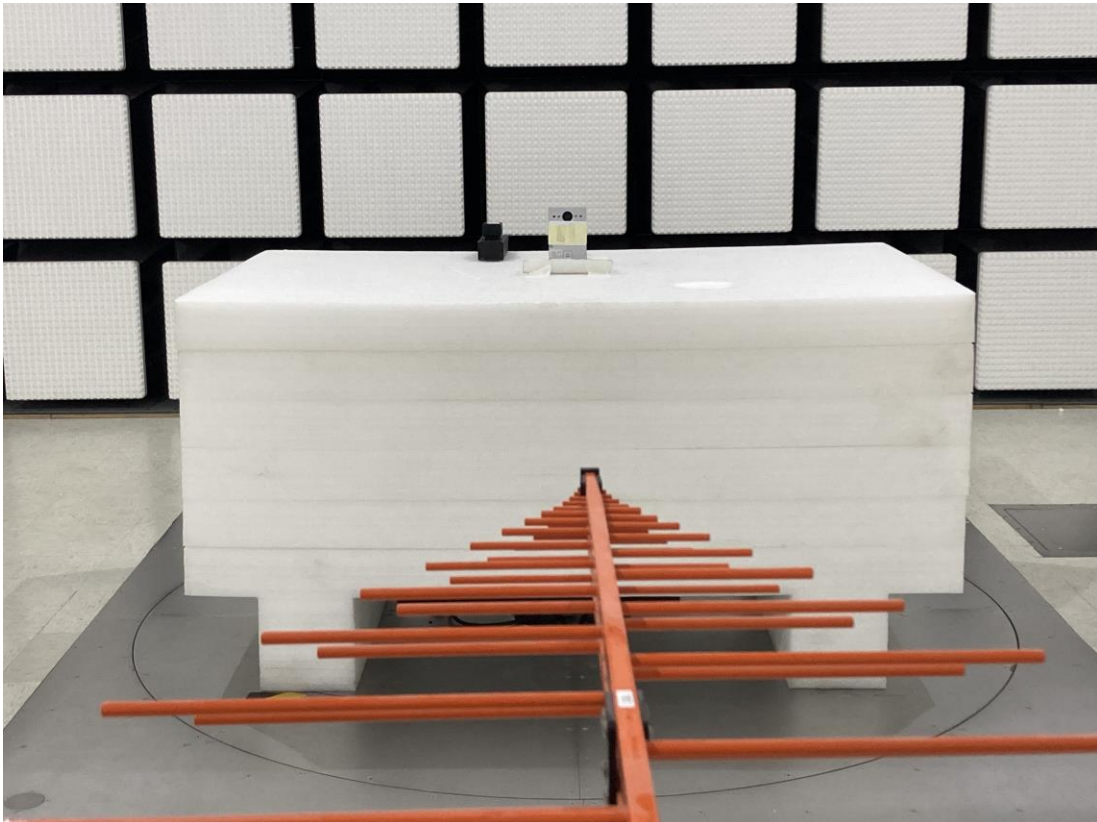
Radiated Emission 30MHz-1GHz View –Adapter mode
