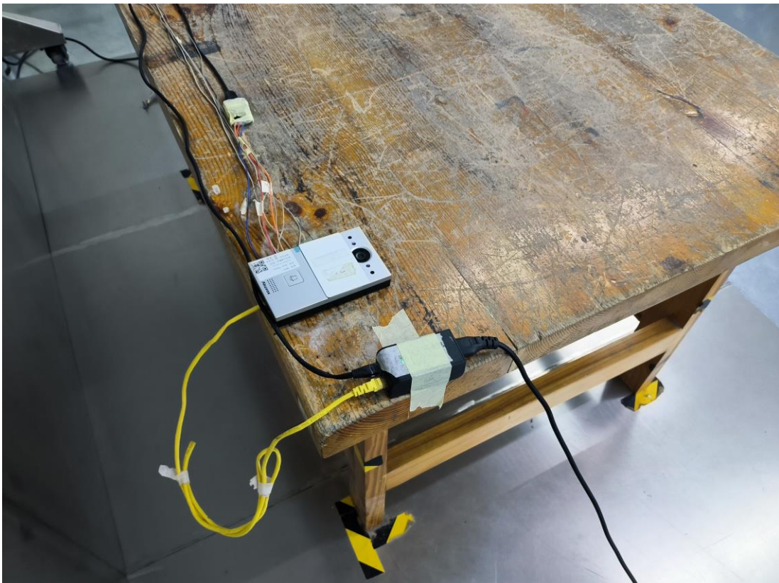
Conducted Emissions Side View –POE mode
