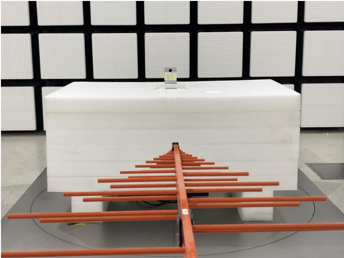
Radiated Emission 30MHz-1GHz View –POE mode
