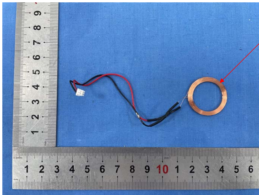
125 kHz Antenna
