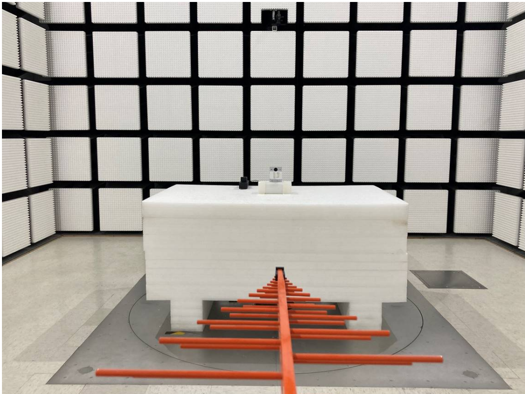
Radiated Emission 30M-1GHz View Adapter
