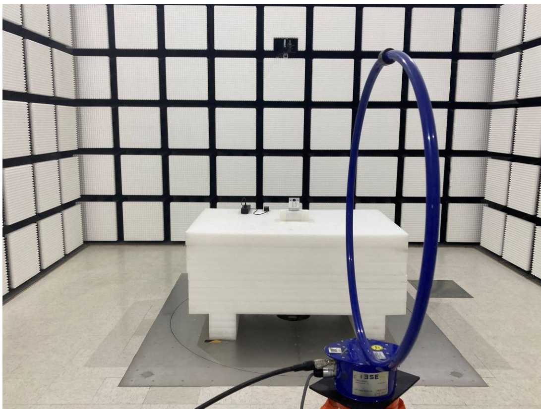
Radiated Emission 9k-30MHz Perpendicular View POE
