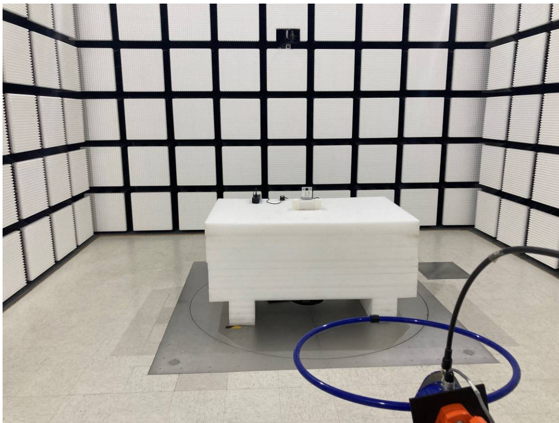
Radiated Emission Below 1GHz View POE
